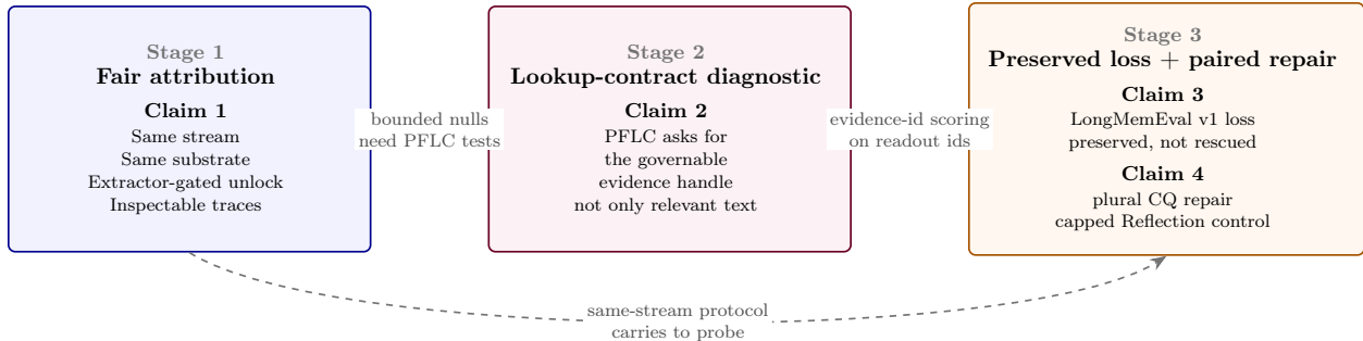
Figure 1: Method-stage view of the four claims. Stage 1 makes policy attribution inspectable by fixing the stream, substrate, and extractor gate. Stage 2 adds PFLC to test whether the governable evidence handle is exposed. Stage 3 preserves the LongMemEval v1 loss and then uses a paired repair and control to pin that loss on answer-time readout cardinality. The figure preserves the claim numbering but frames the contribution as an attribution method.
