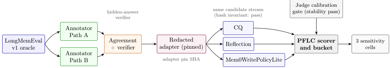
Figure 4: Controlled LongMemEval externalization. The v1 oracle source is annotated by two independent paths whose agreement is verified before any policy sees data. The redacted adapter strips the gold answer, pins a SHA-locked candidate stream, and feeds the same stream to every policy. The judge calibration gate must clear stability before scoring runs; the PFLC scorer reads policy outputs across three contract-sensitivity cells.
