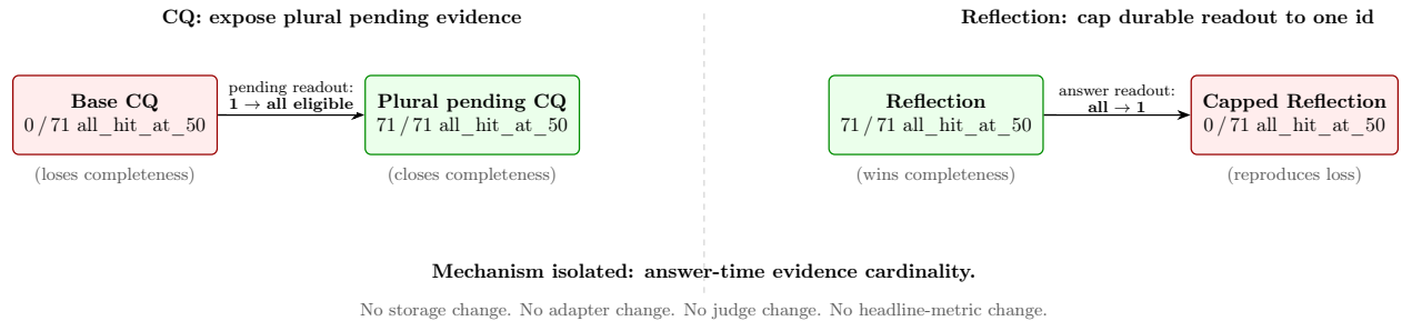
Figure 7: Cardinality-repair follow-up. Changing the CQ pending-readout cardinality from singleton to plural converts a 0/71 loss into a 71/71 win on all_hit_at_50 in the primary cell. Capping the durable Reflection readout to a single id reproduces the original CQ loss with the same magnitude. The symmetric swap isolates answer-time evidence cardinality as the responsible interface variable; nothing else in the pipeline changes.
