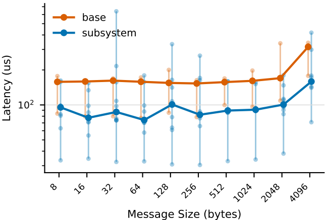
OSU allreduce (arm64)
