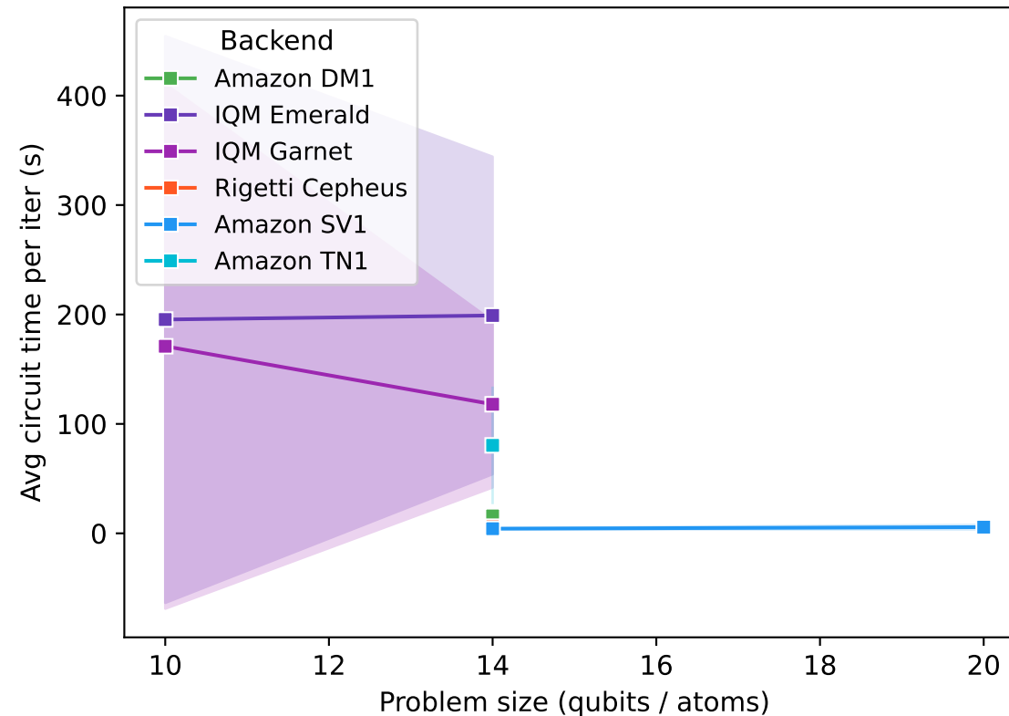
Circuit time (submit→result) vs. problem size
