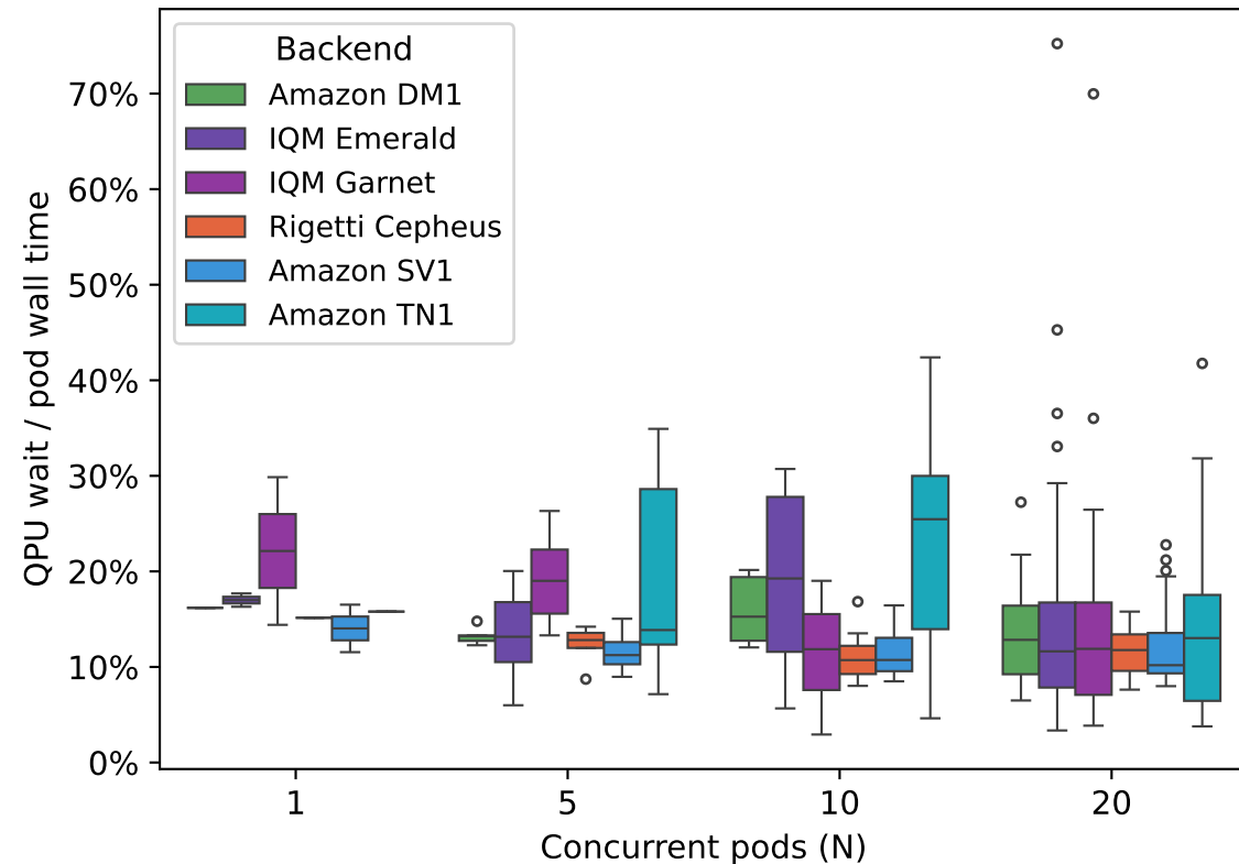
Classical idle fraction vs. concurrency
