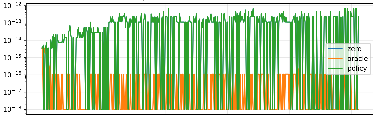
Expected oracle Bellman residual
