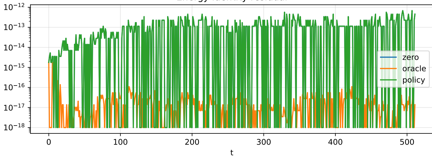
Energy identity residual
