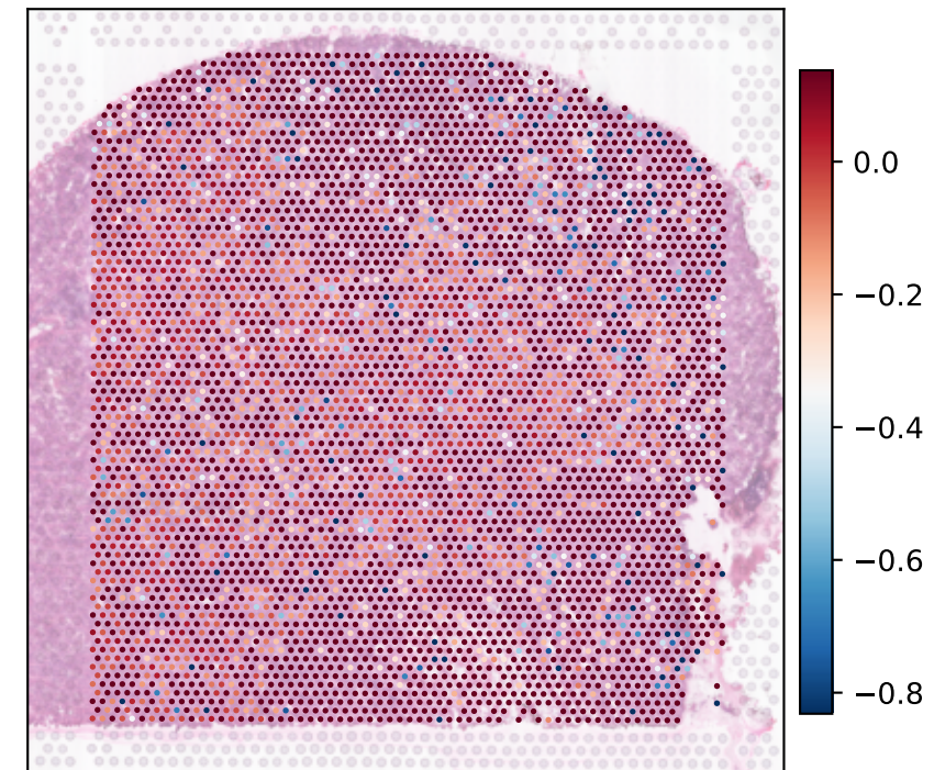
DM1_like_score (= -RAI_8)
