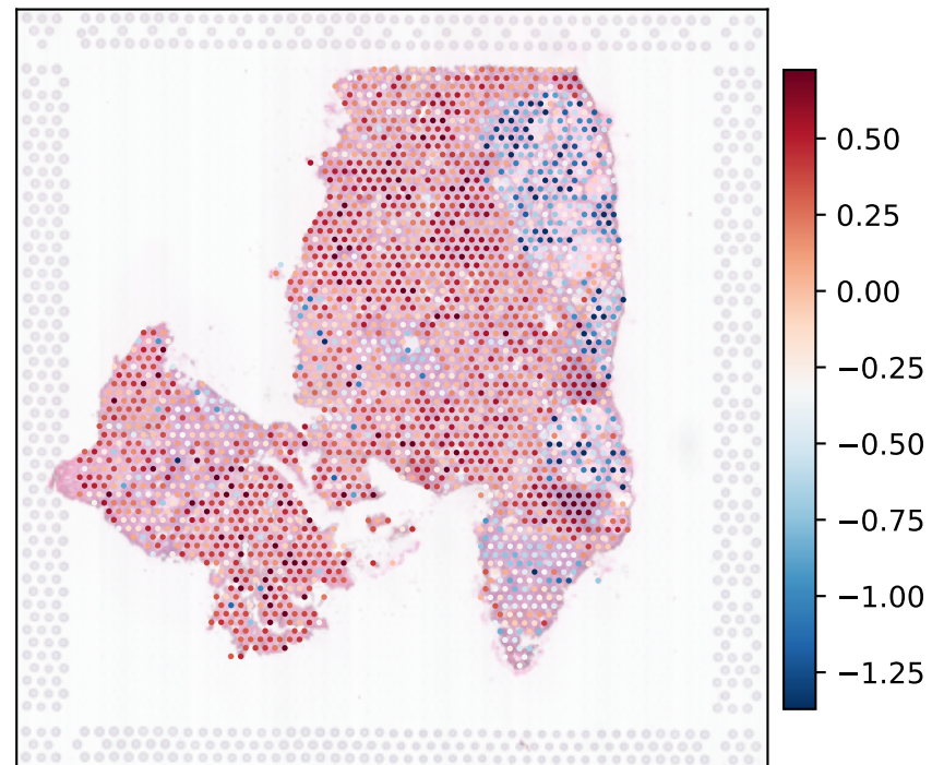
DM1_like_score (= -RAI_8)
