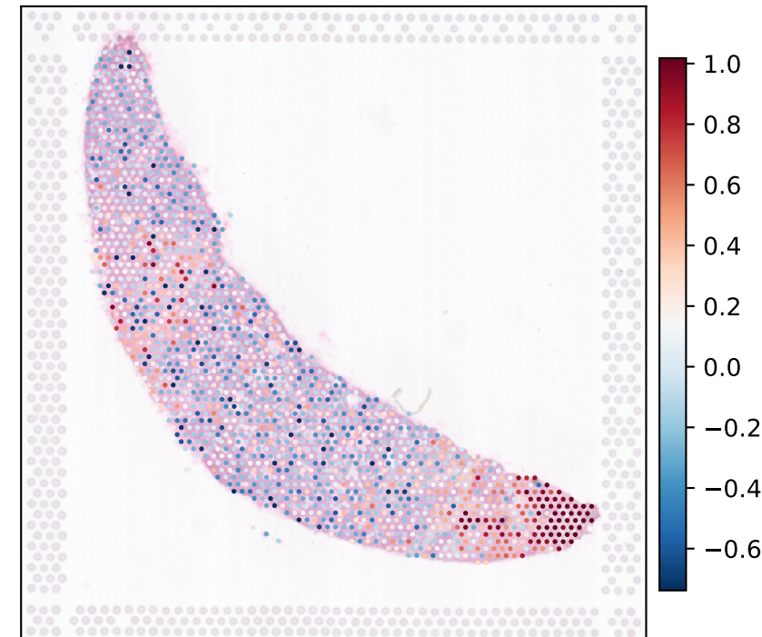
DM1_like_score (= -RAI_8)
