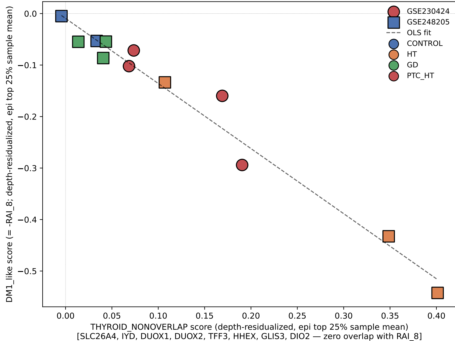
Supp Fig X2 — Cross-validation against independent thyroid-lineage axis All 12 external samples · Spearman \rho = -0.94 ( p = 7.0\text{e-}06 ) · Pearson r = -0.98 ( p = 6.6\text{e-}09 )
