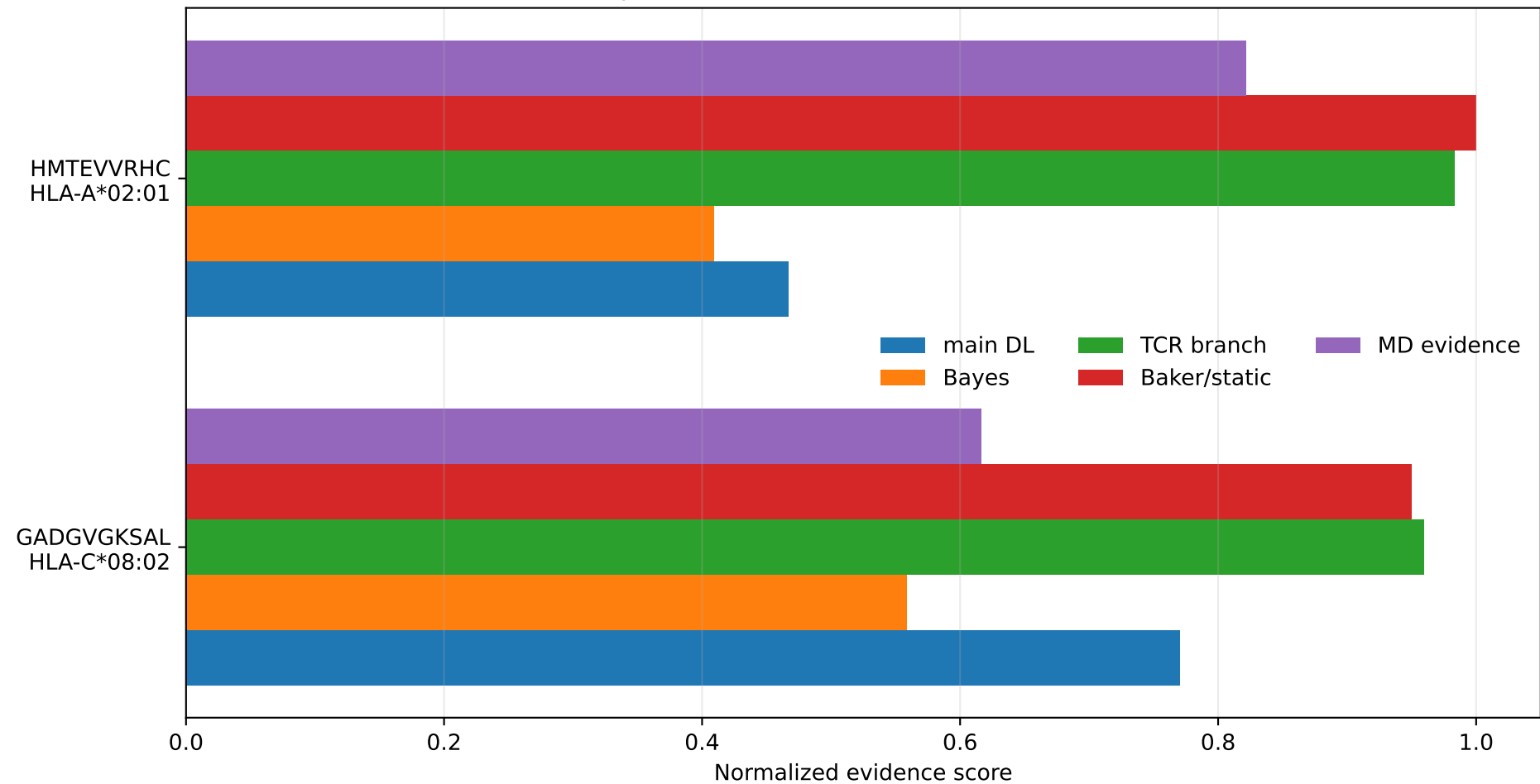
Representative candidate evidence board
