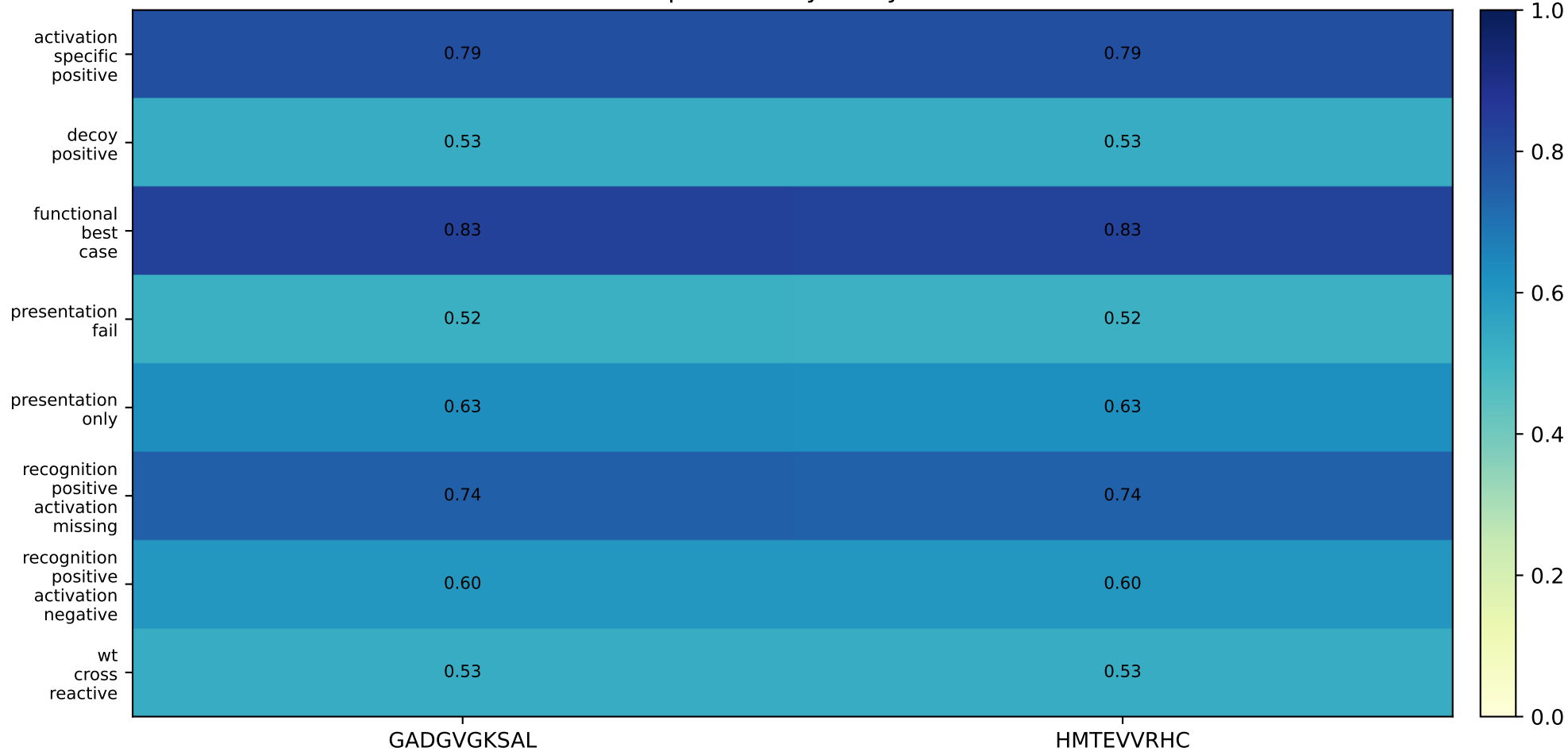
What-if posterior by assay scenario
