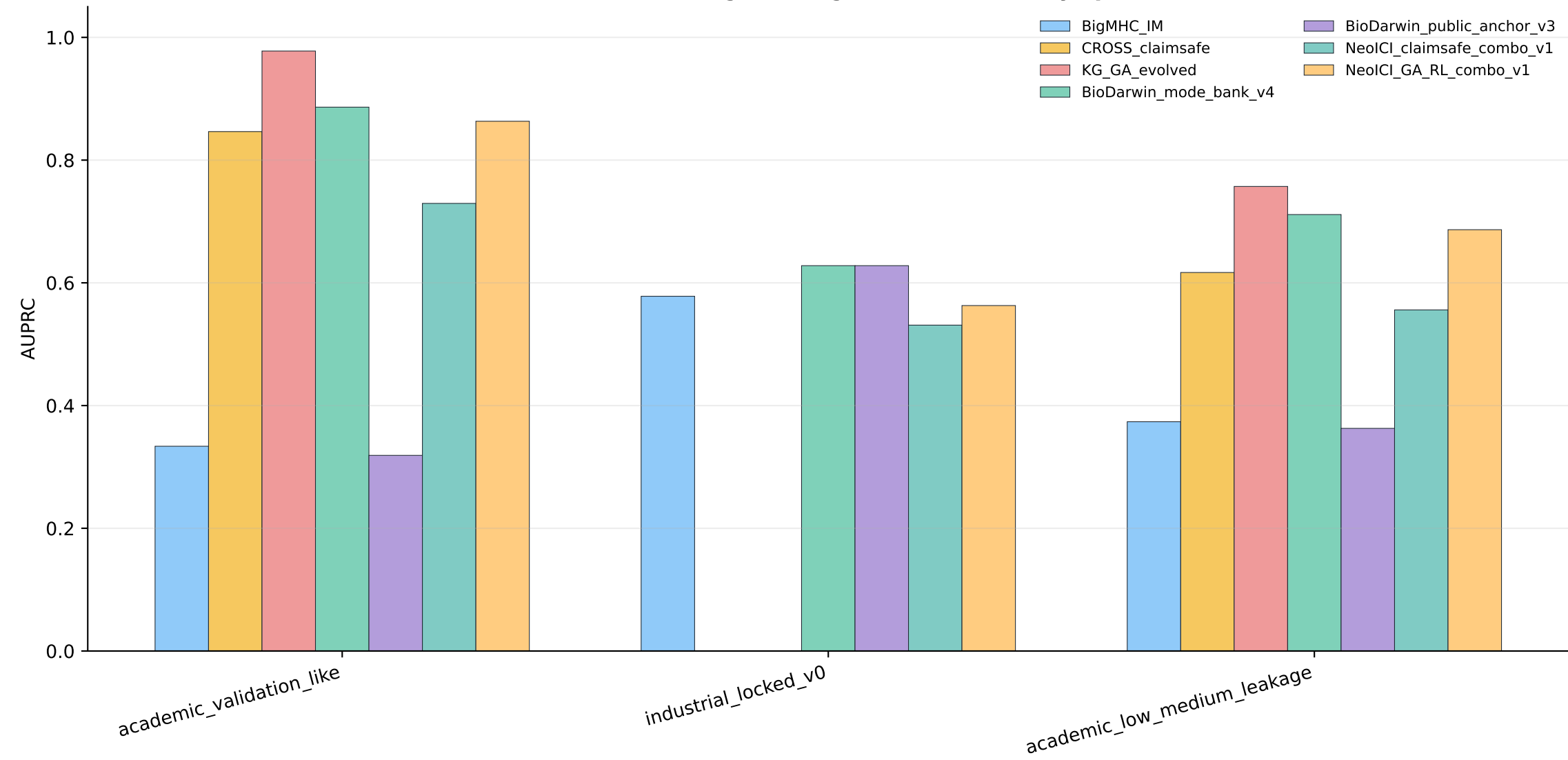
NeolCI-combo algorithm gauntlet: AUPRC by split
