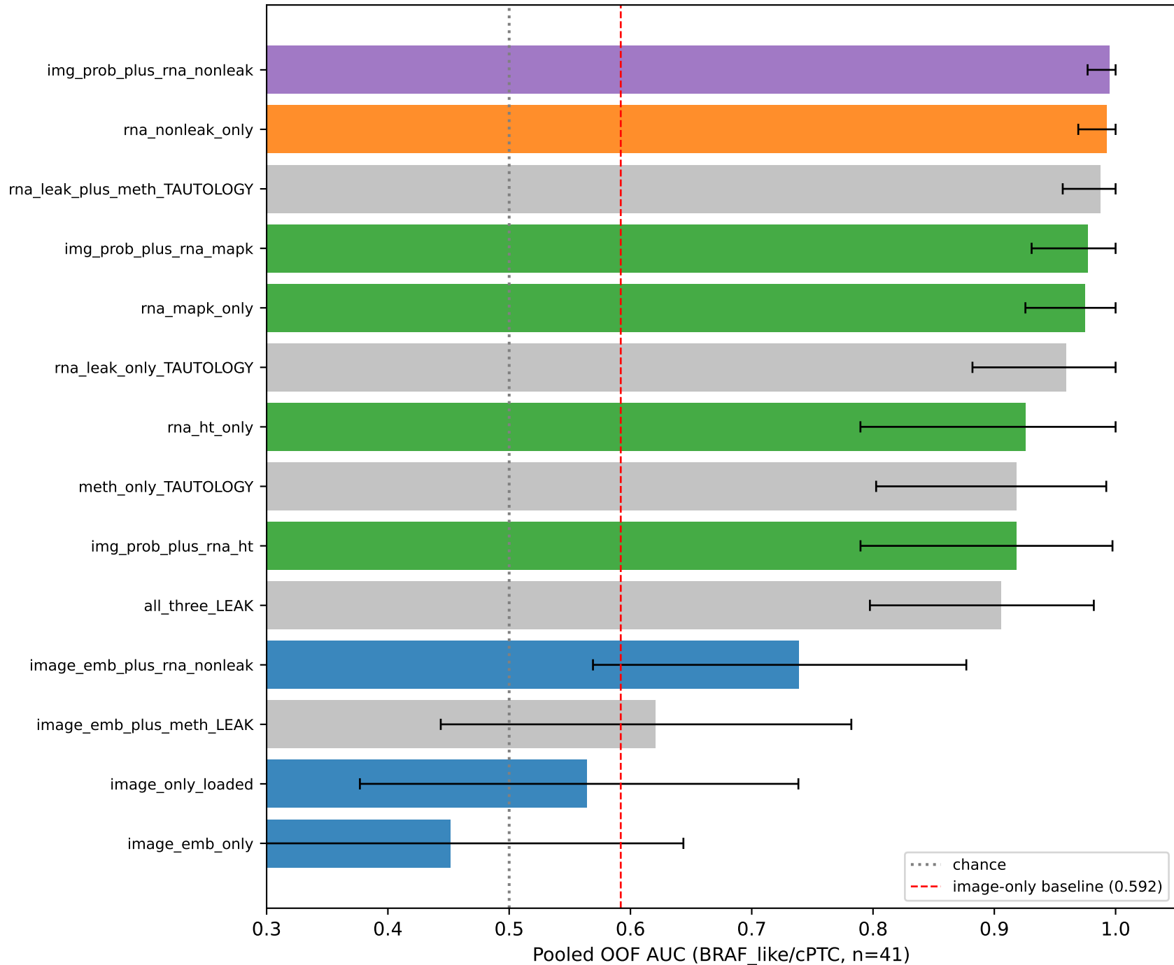
Paper 2 BRAF_like/cPTC multimodal rescue 5-fold CV (same folds as image-only); 95% CI = stratified bootstrap (1000) Gray = label-leaking (HM450 8-gene panel defines DM1/DM2)
