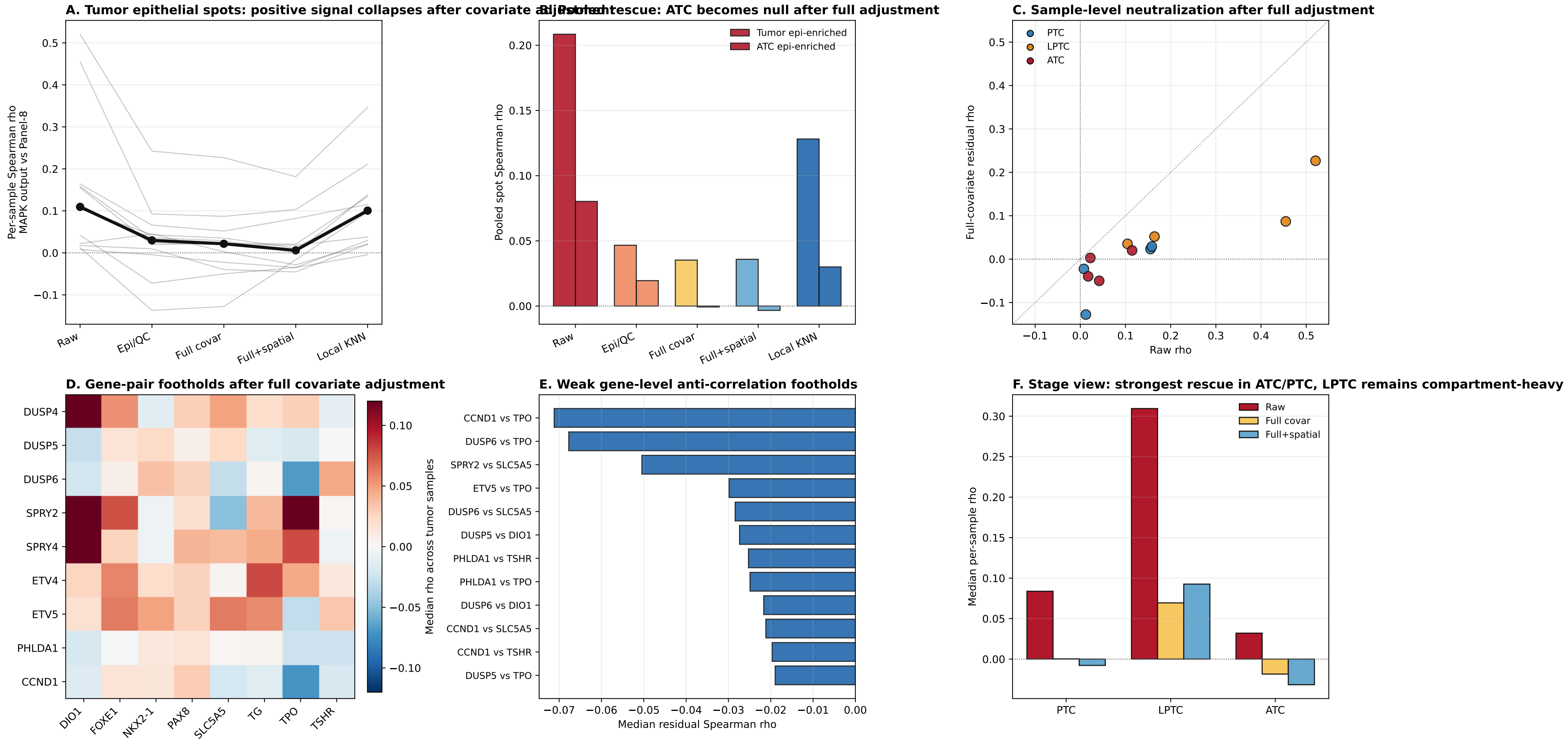
Figure SX_v16. Spatial MAPK-panel failure autopsy: the Visium module signal is mostly compartment/QC/spatial structure, not a usable anti-correlation test.
