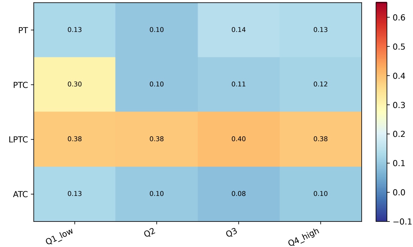
B. Spatial rho by within-slide epithelial-score quartile
