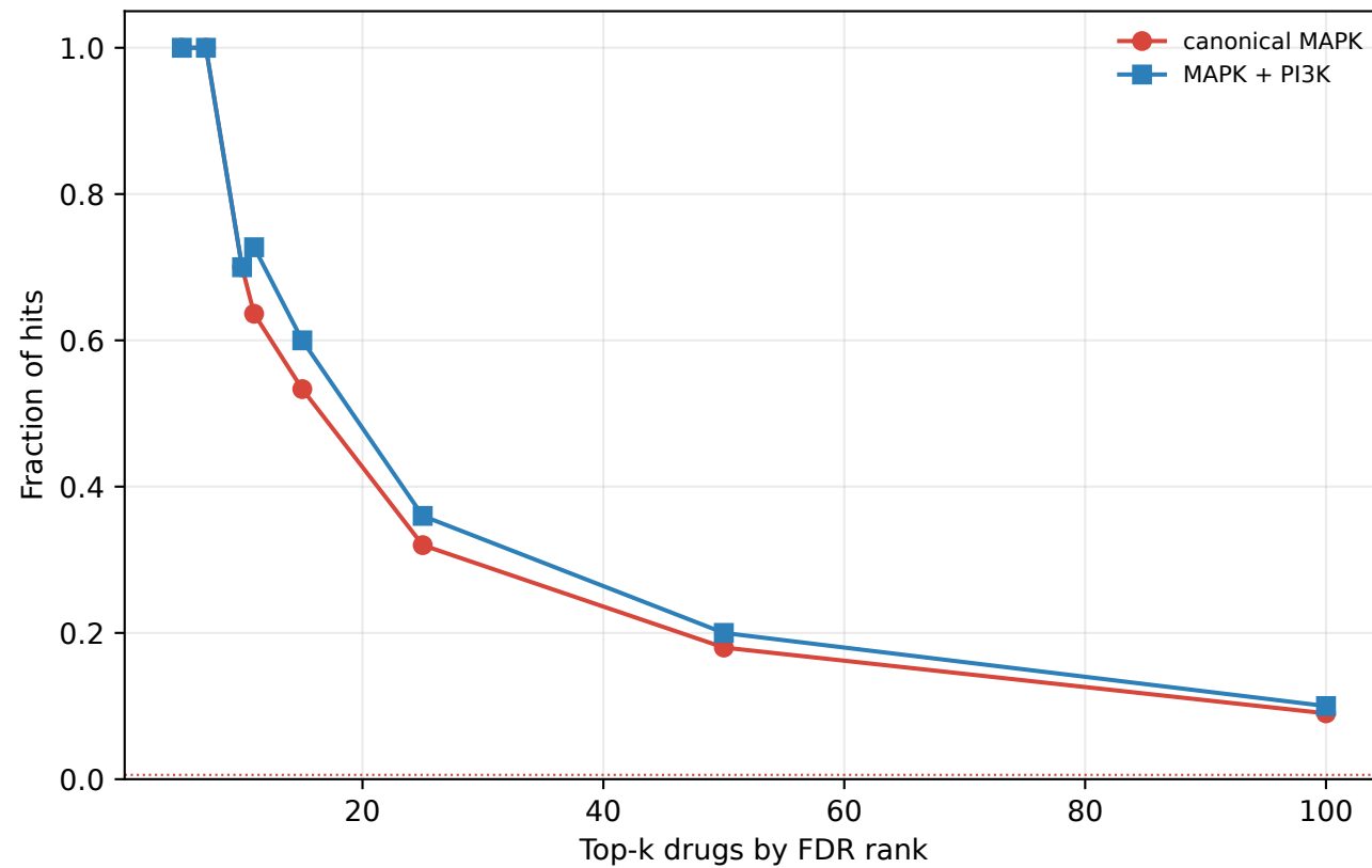
C. PRISM enrichment: top 7 all MAPK, top 15 not all MAPK
