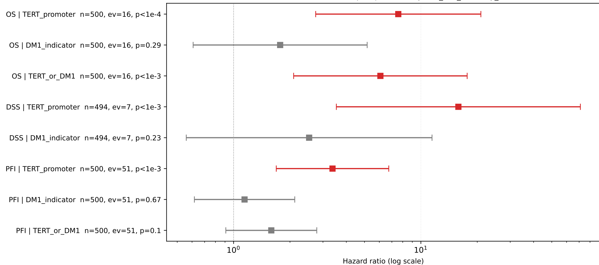
TCGA-THCA TERT × DM × OS/DSS/PFI Cox HR — Round 3 (2026-05-08) (36 recovered TERT+ samples per memory v17_tert_recovery_v2)
