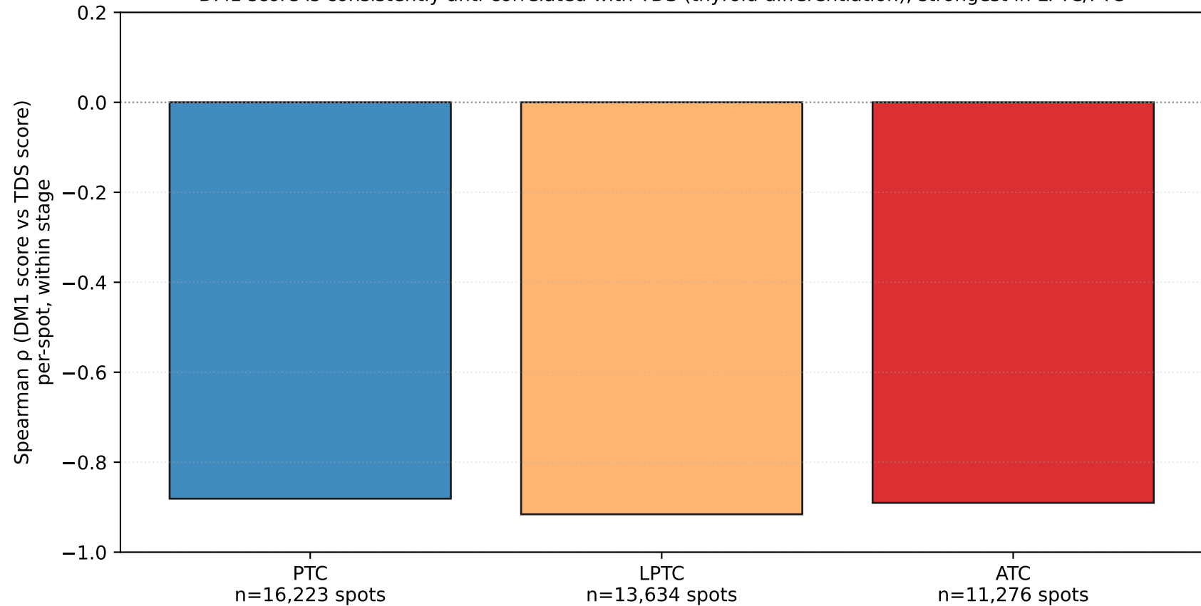
Spatial DM1 \leftrightarrow TDS niche correlation by stage (GSE250521 Visium) DM1 score is consistently anti-correlated with TDS (thyroid differentiation), strongest in LPTC/PTC
