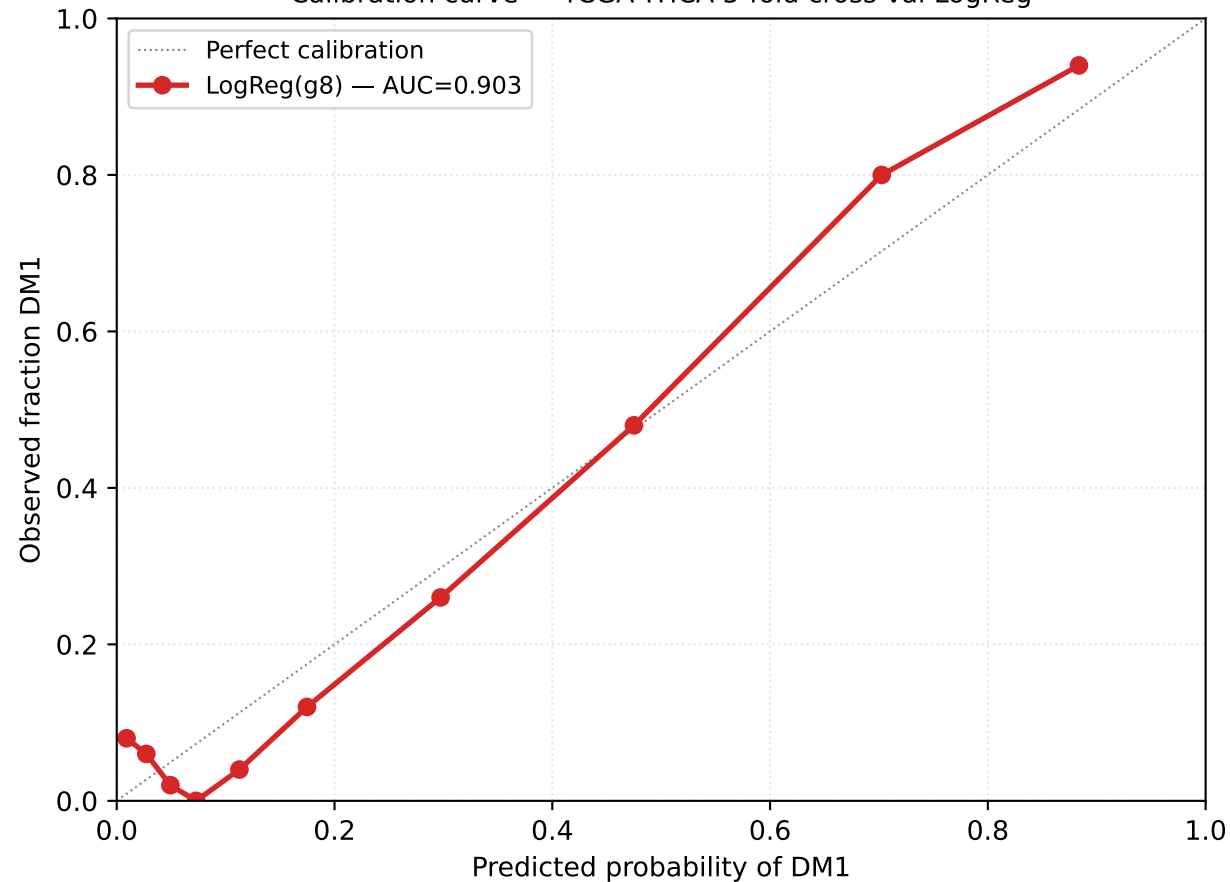
Calibration curve — TCGA-THCA 5-fold cross-val LogReg
