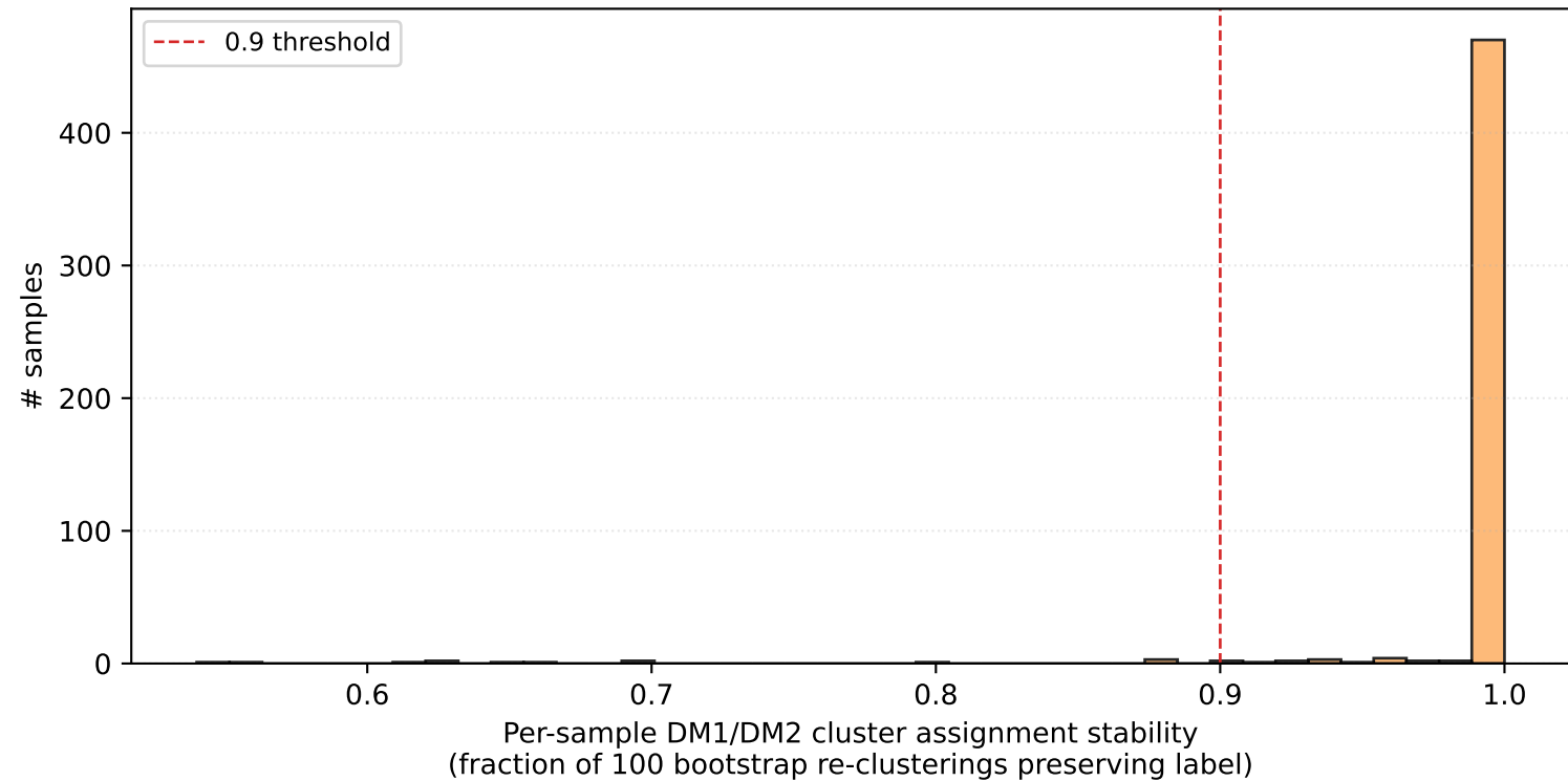
DM1/DM2 cluster stability bootstrap — TCGA-THCA n=500 mean stability=0.990; 97% of samples \geq 0.9 stability
