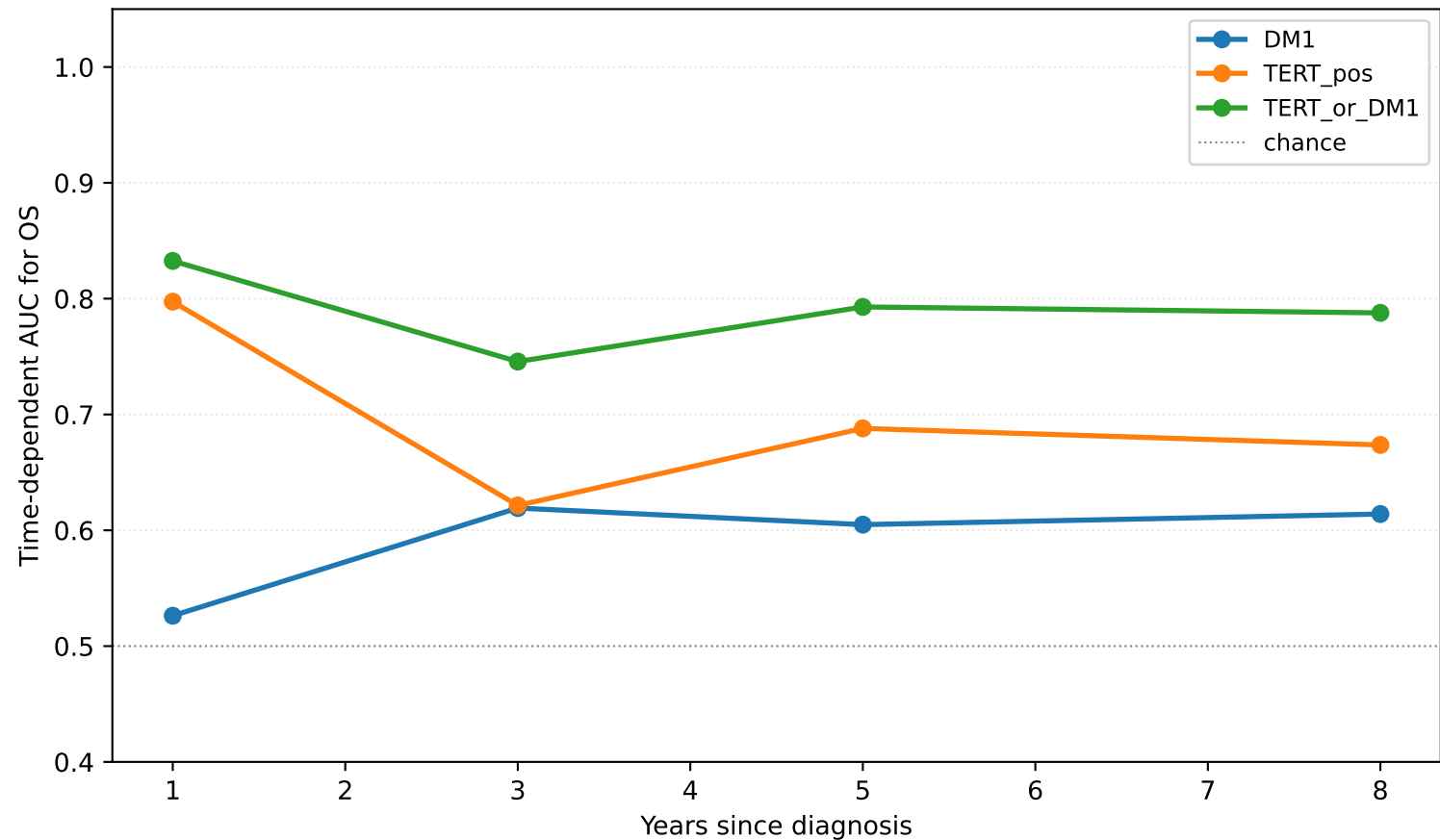
TCGA-THCA time-dependent ROC AUC for OS — DM1 + TERT
