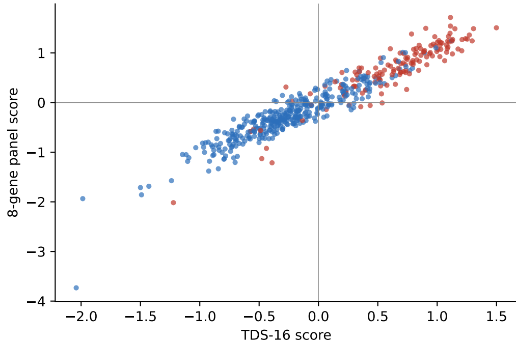
score correlation (Spearman \rho = 0.954 )
