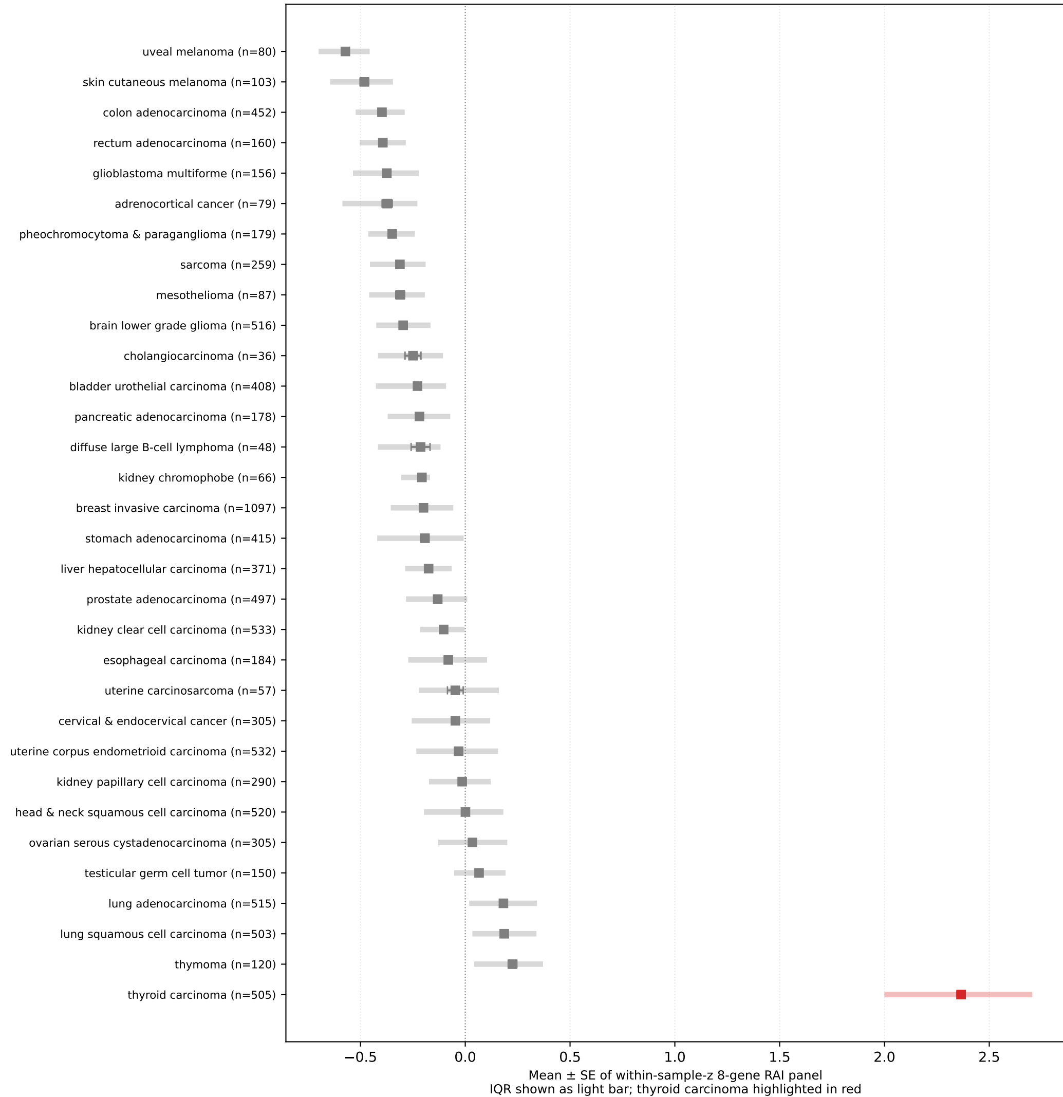
DM1 8-gene panel cross-cancer specificity (TCGA pan-cancer n=10,593 primary tumors) Thyroid uniquely retains coordinated 8-gene panel expression — DM panel is thyroid-specific by design
