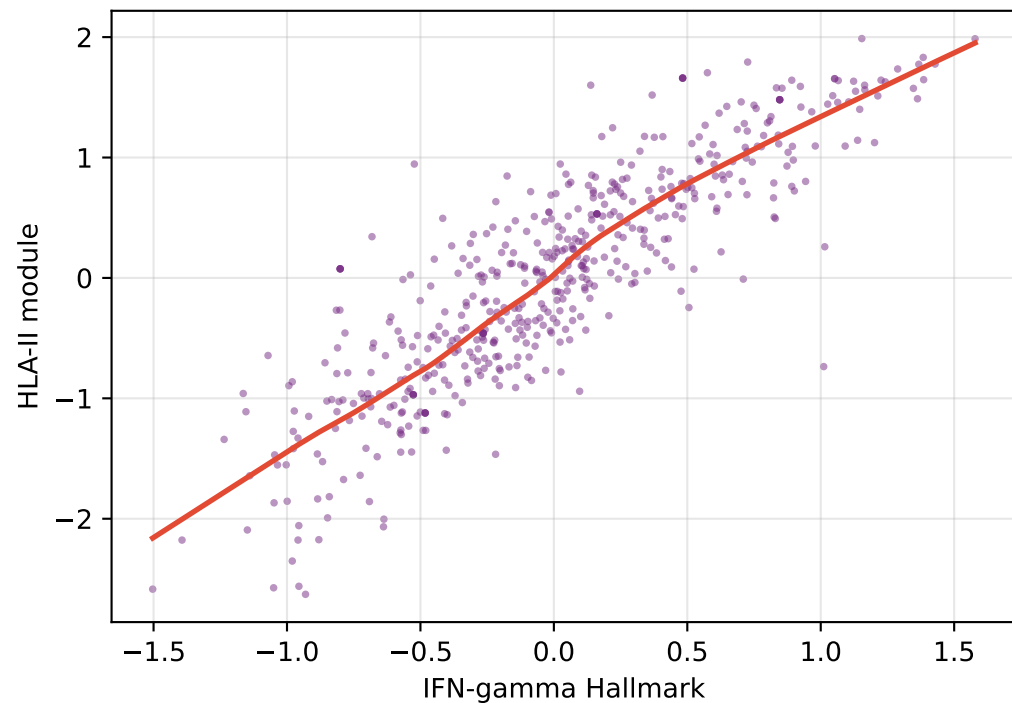
IFN-gamma Hallmark vs HLA-II module Spearman rho=0.873, p=2.00e-165, n=527
