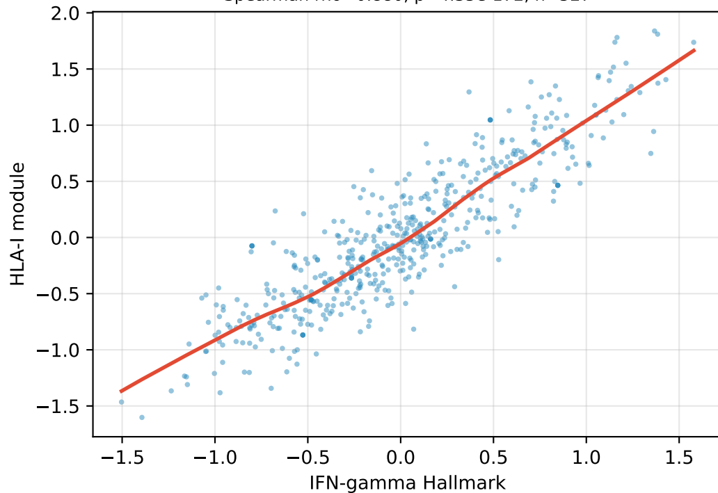
IFN-gamma Hallmark vs HLA-I module Spearman rho=0.880, p=4.35e-172, n=527
