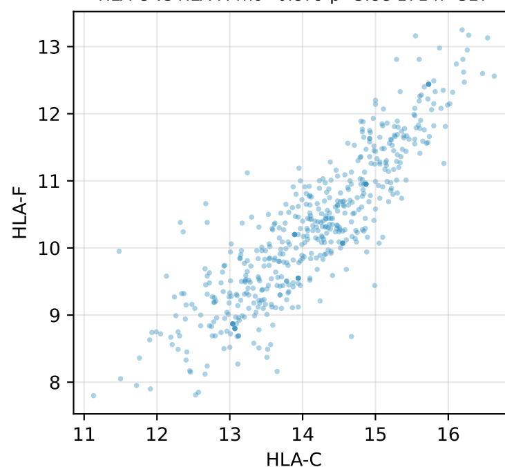
HLA-C vs HLA-F: \rho=0.879 p=5.8e-171 n=527
