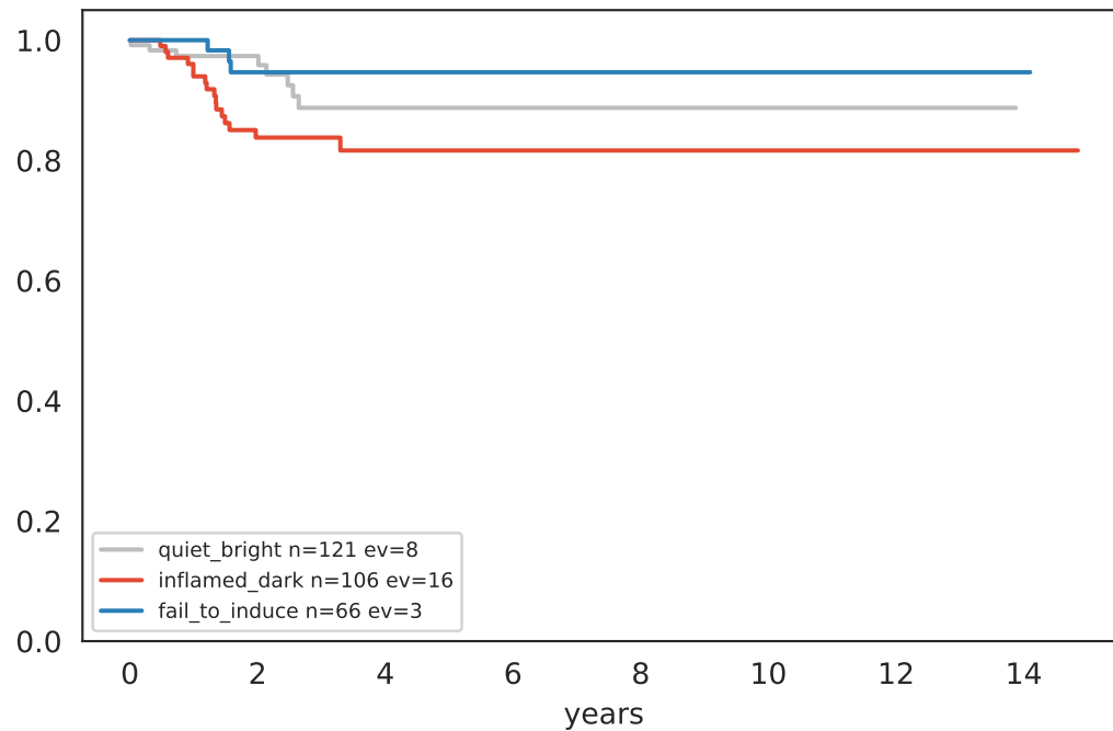
DFI by quadrant (TCGA-THCA)
