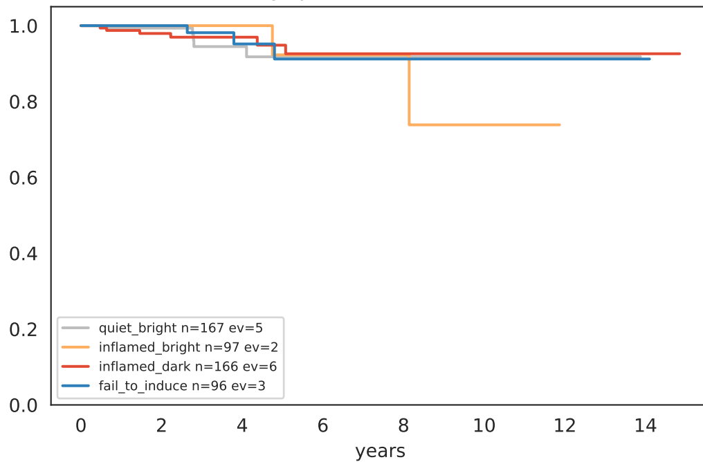
PFI by quadrant (TCGA-THCA)
