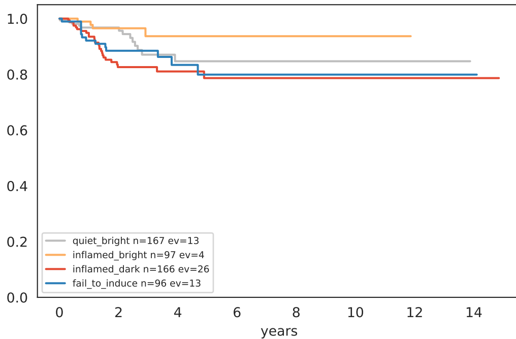
PFI by quadrant (TCGA-THCA)
