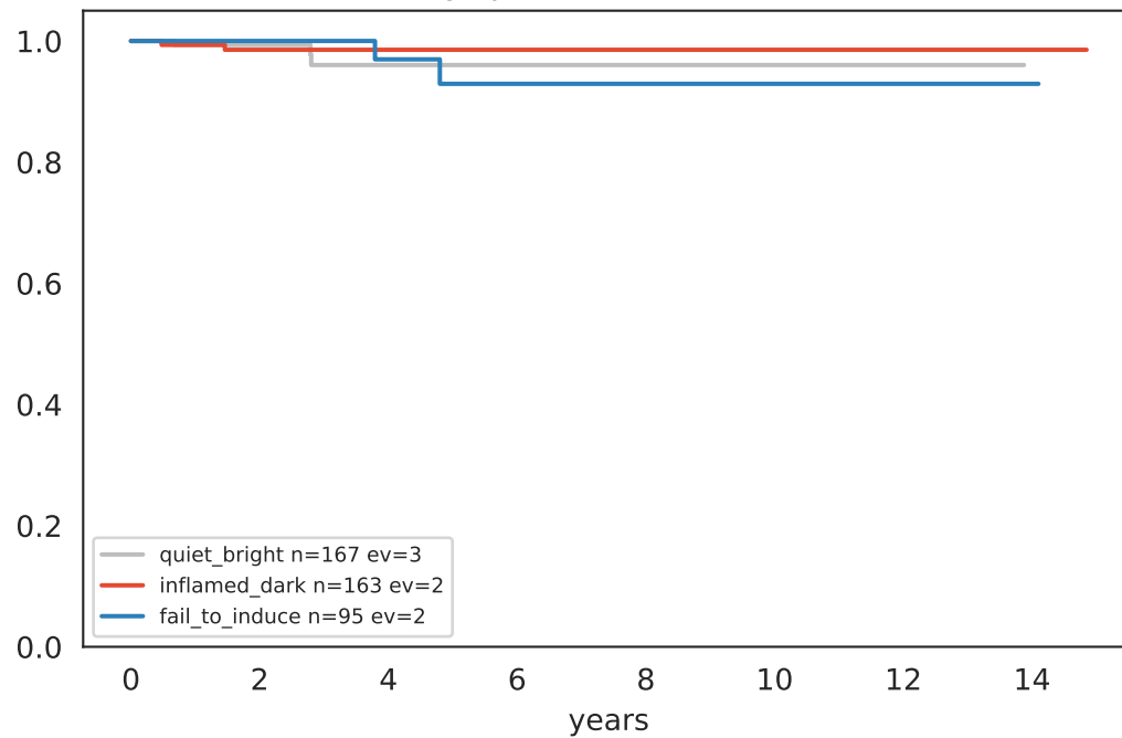
DFI by quadrant (TCGA-THCA)
