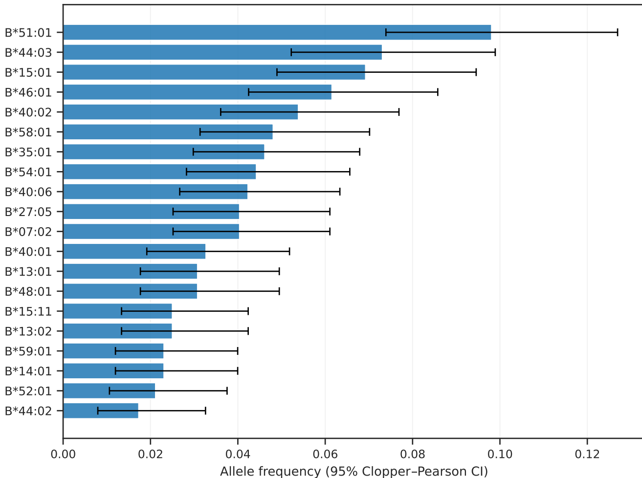
K2 PRJEB11591 — HLA-B top-20 alleles (N=260 typed)
