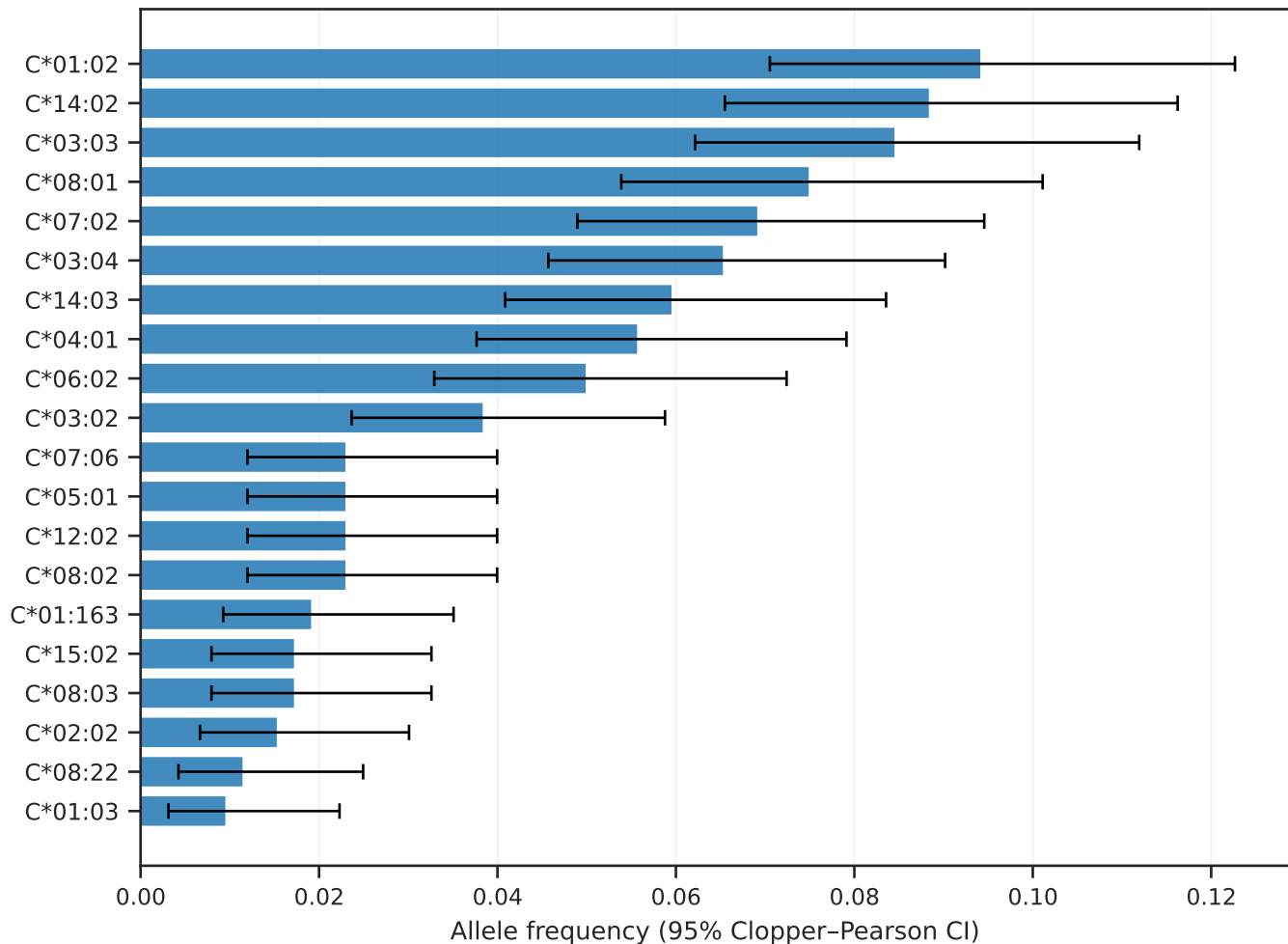
K2 PRJEB11591 — HLA-C top-20 alleles (N=260 typed)
