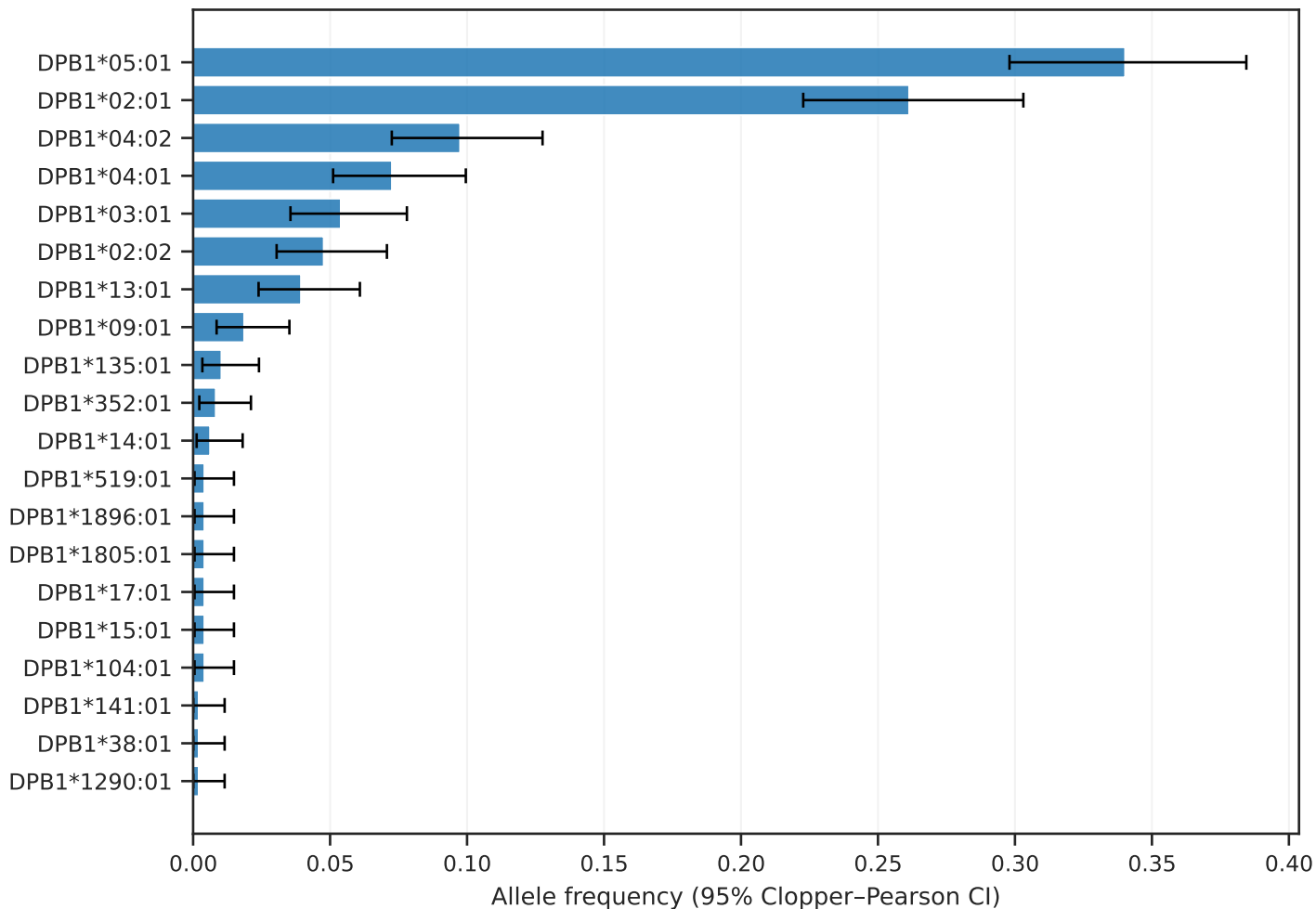
K2 PRJEB11591 — HLA-DPB1 top-20 alleles (N=241 typed)
