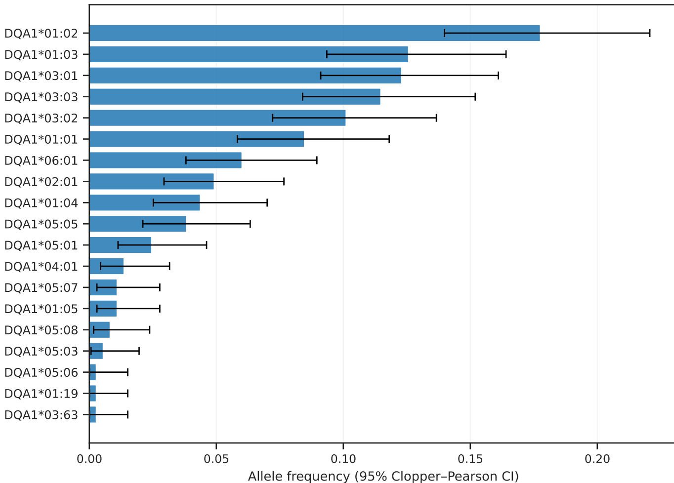
K2 PRJEB11591 — HLA-DQA1 top-20 alleles (N=183 typed)
