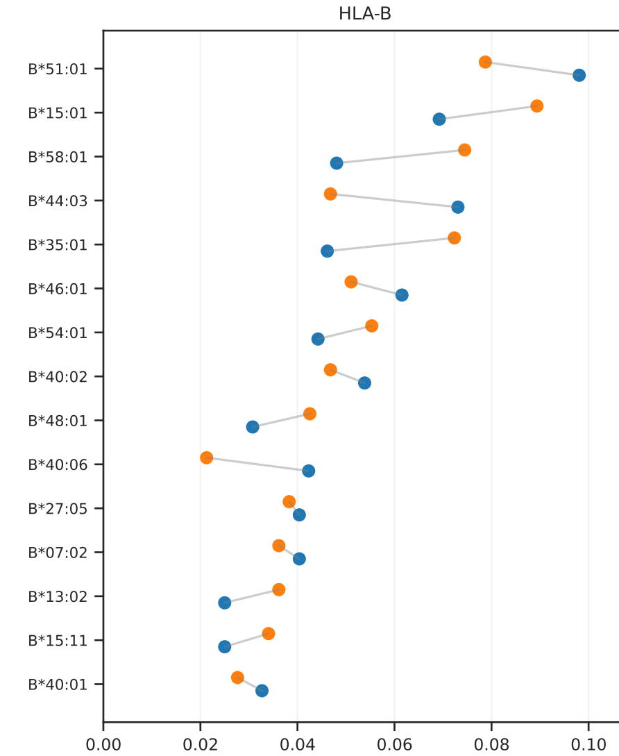
K2 vs Lee 2024 (normal-only) — per-locus top-15 allele forest (both Korean RNA-seq, arcasHLA)
