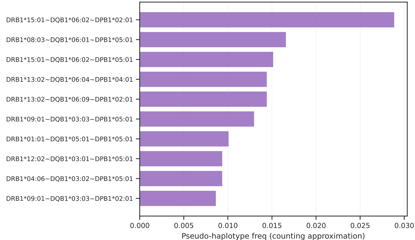
Class-II DRB1~DQB1~DPB1 top-10
