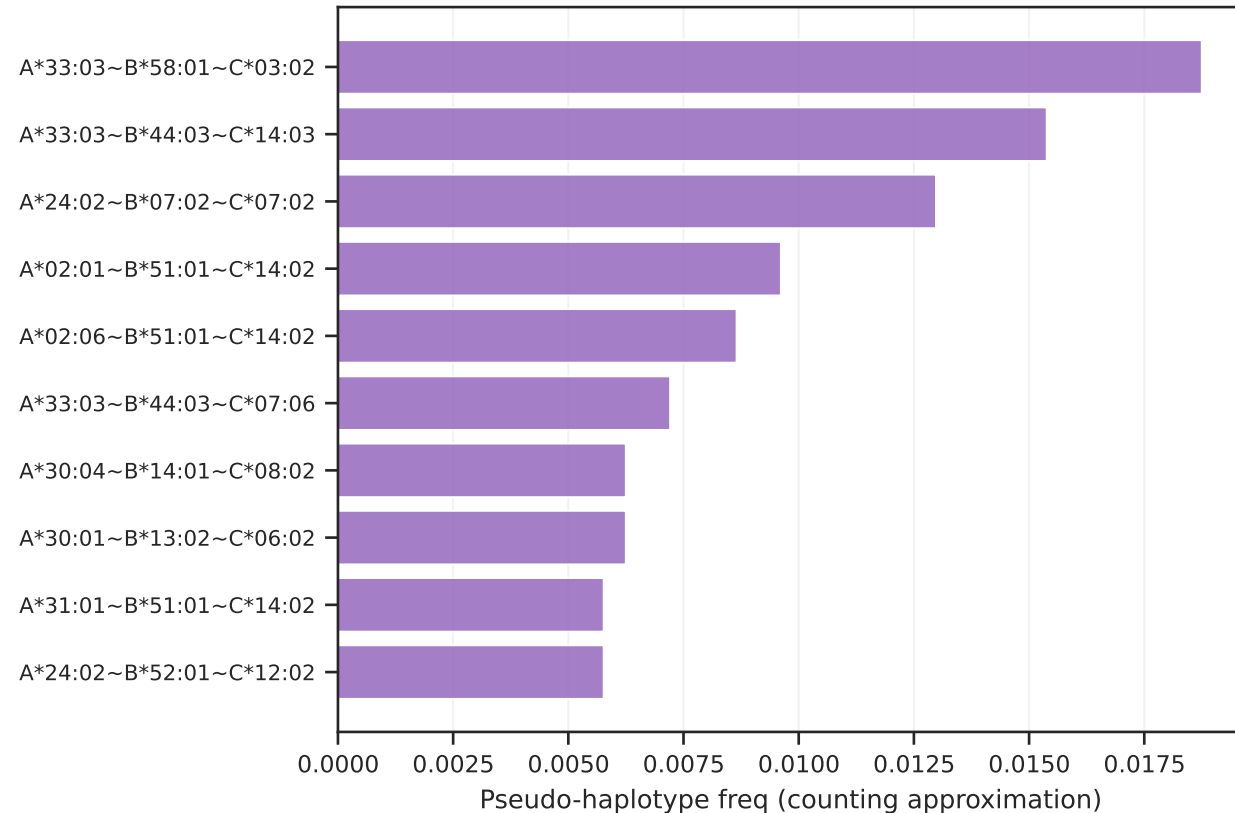
Class-I A~B~C top-10
