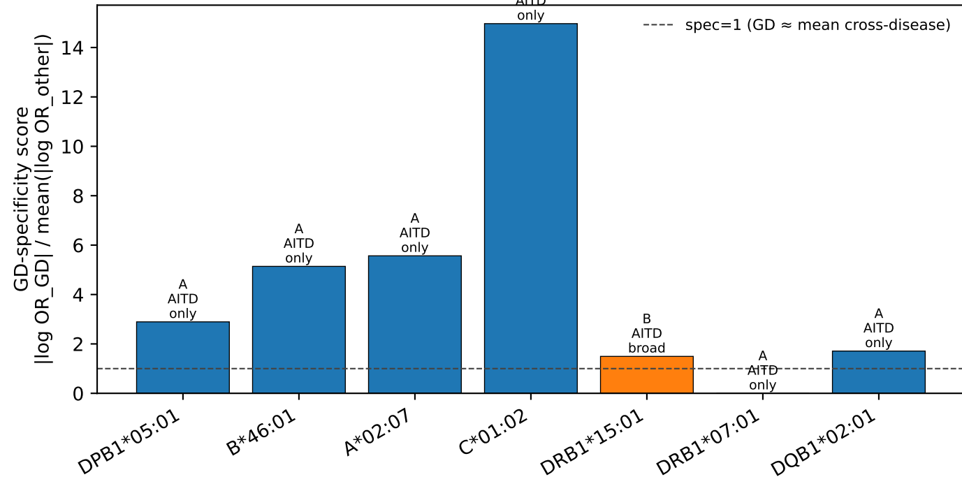
Track 31 F06 — GD-specificity of Track 1 focus alleles (>1 = GD-concentrated; ~1 = comparable; <1 = broader autoimmune signal)
