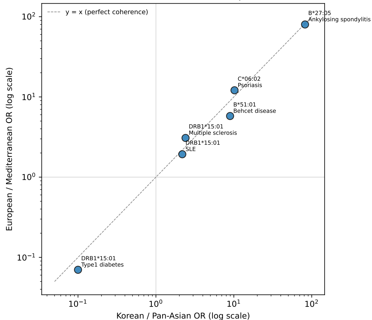
Track 31 F08 — Korean vs trans-ancestry coherence
