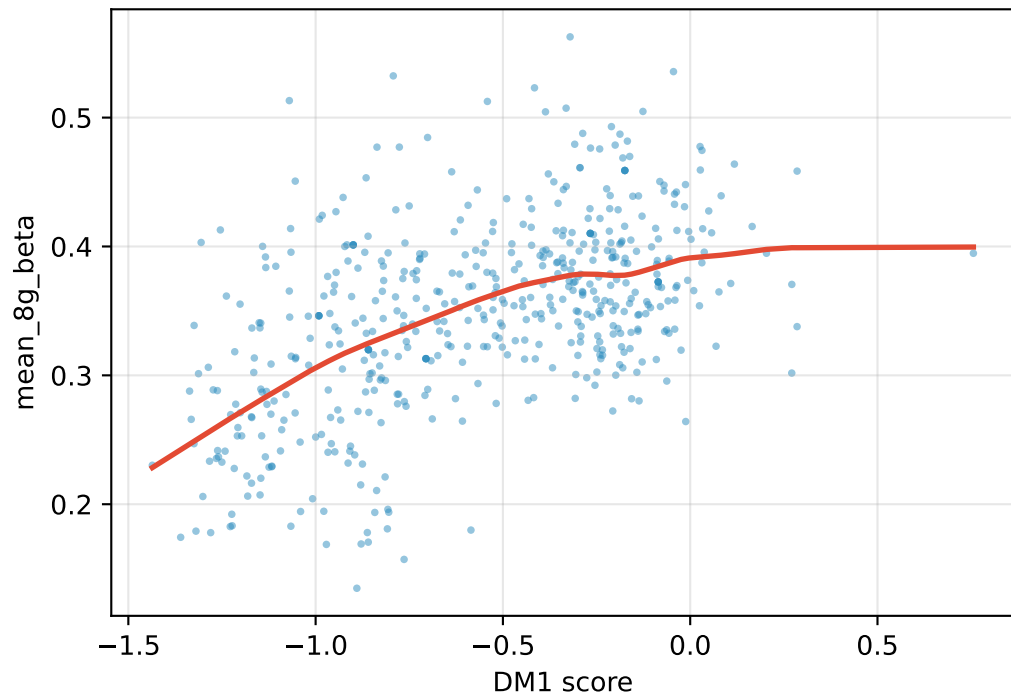
DM1 vs mean_8g_beta Spearman rho=0.491, p=5.09e-33, n=523
