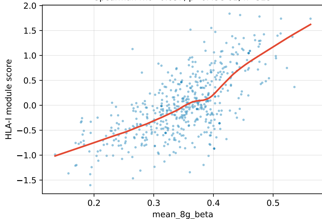
mean_8g_beta vs HLA-I module Spearman rho=0.637, p=6.45e-61, n=523
