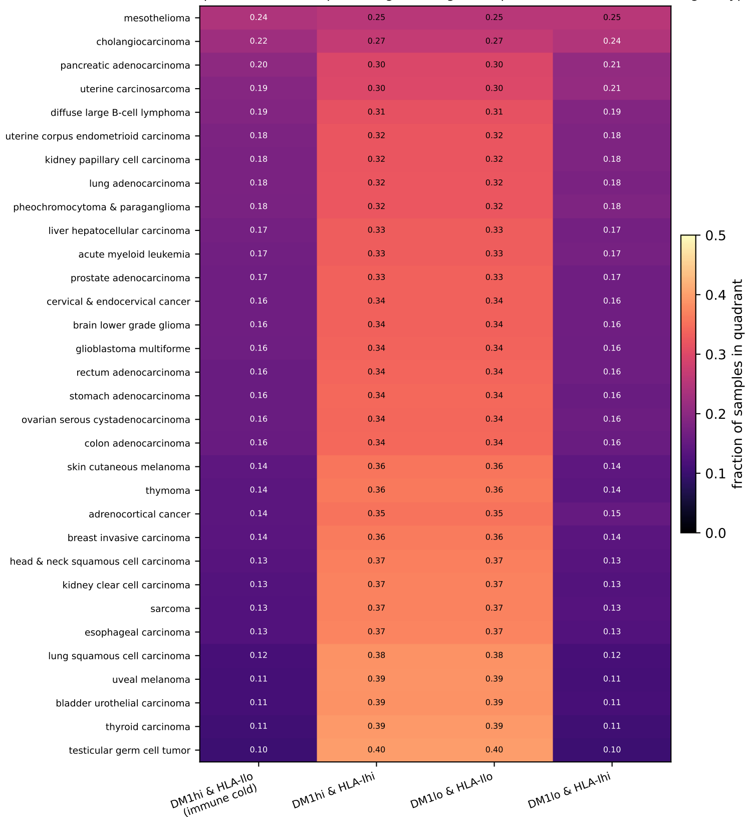
DM1 x HLA-I quadrant fractions per lineage - HLA gene-expression module - not allele genotype.
