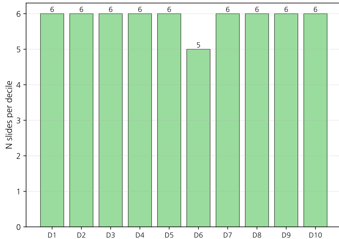
(B) Decile sample sizes
