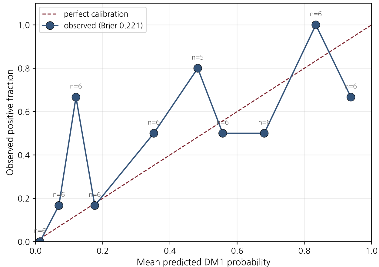
(A) Reliability diagram (10 deciles) · HL p=1.8e-04
