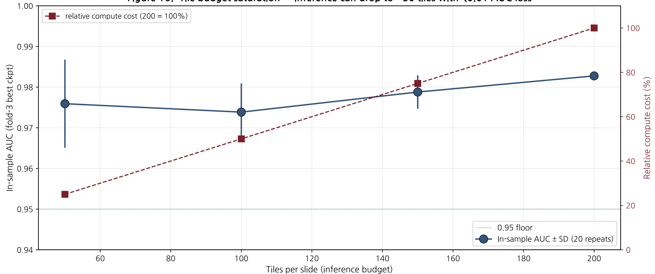
Figure 16. Tile budget saturation — inference can drop to ~50 tiles with <0.01 AUC loss
