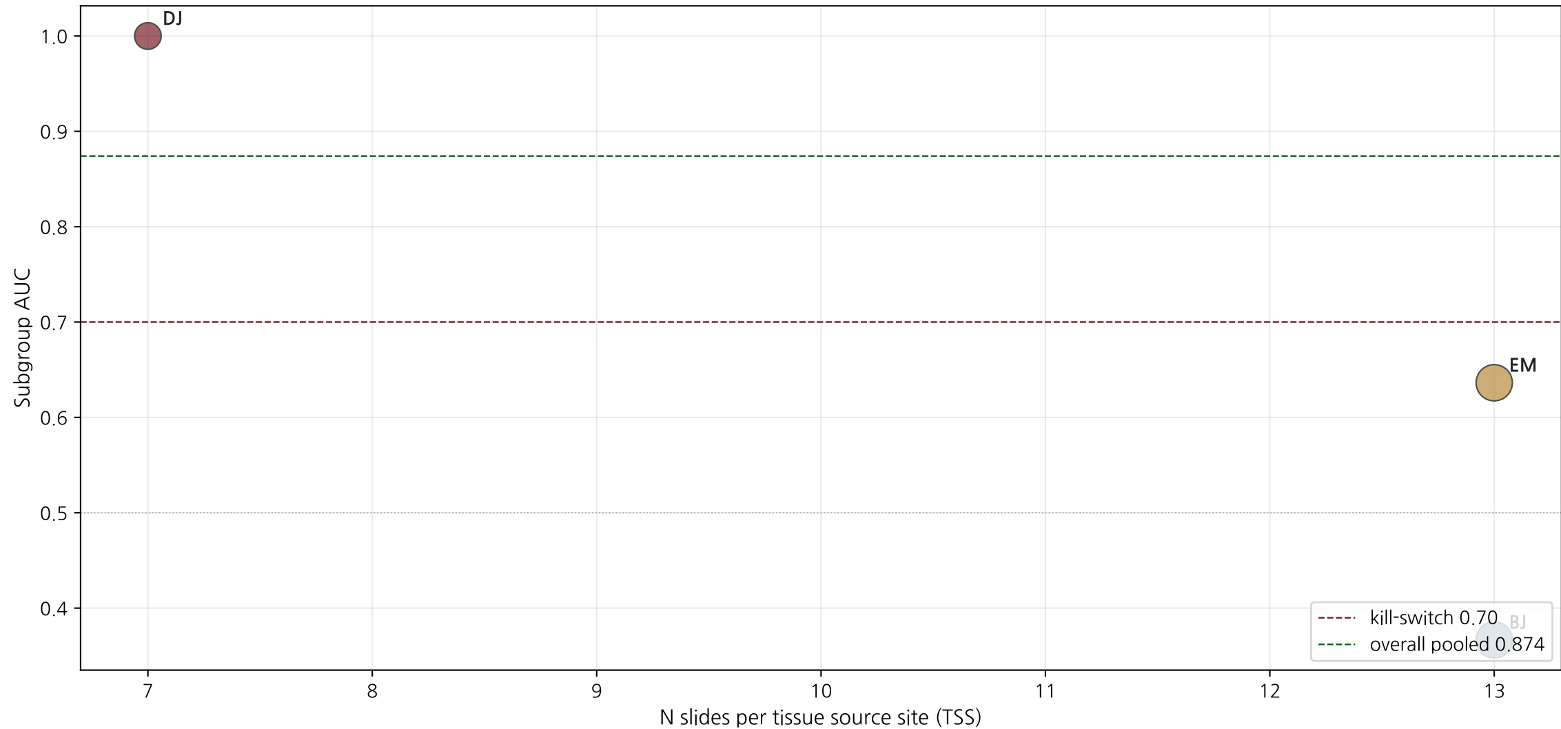
Figure 20. Tissue source site (TSS) heterogeneity — bubble size = N
