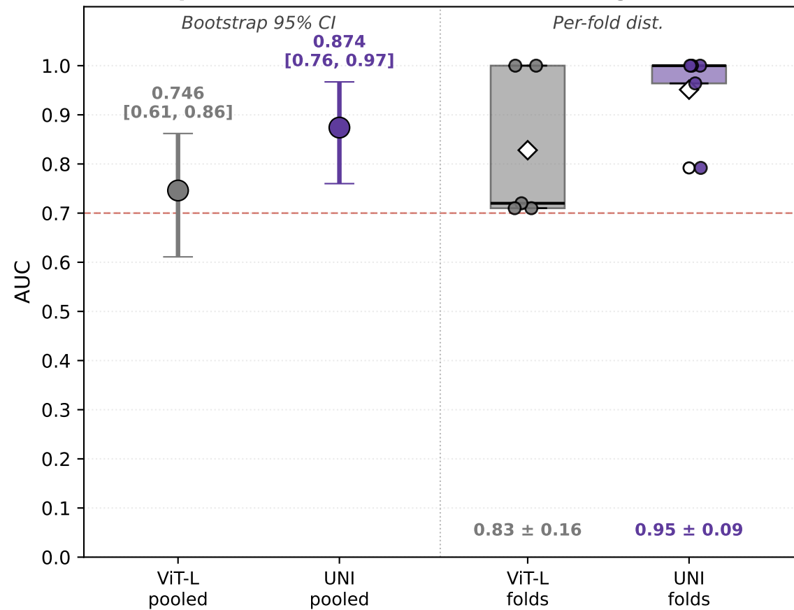
B. UNI provides \Delta AUC = +0.128 over ImageNet ViT-L
