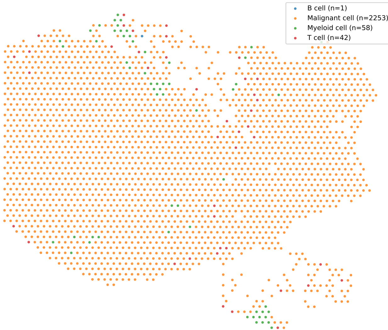
Mapped celltype — ATC-2
