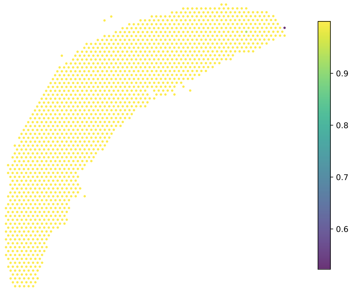
Mapping confidence
