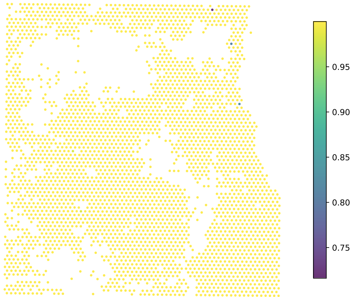
Mapping confidence
