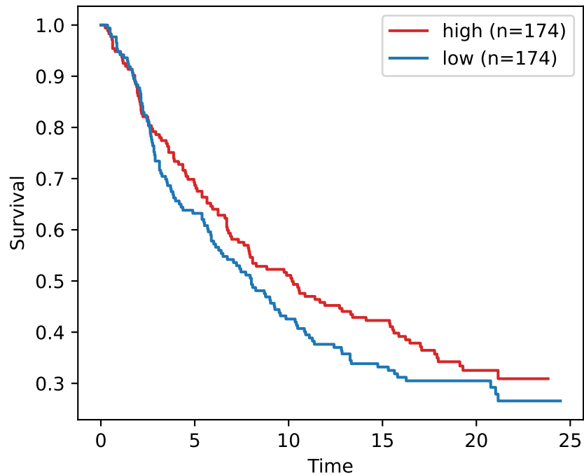
IMvigor210 — DM1_inflam median split (logrank p=0.255)
