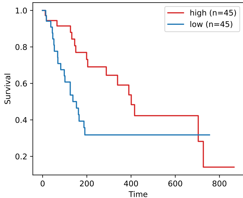
GSE176307 — DM1_inflam median split (logrank p=0.0329)
