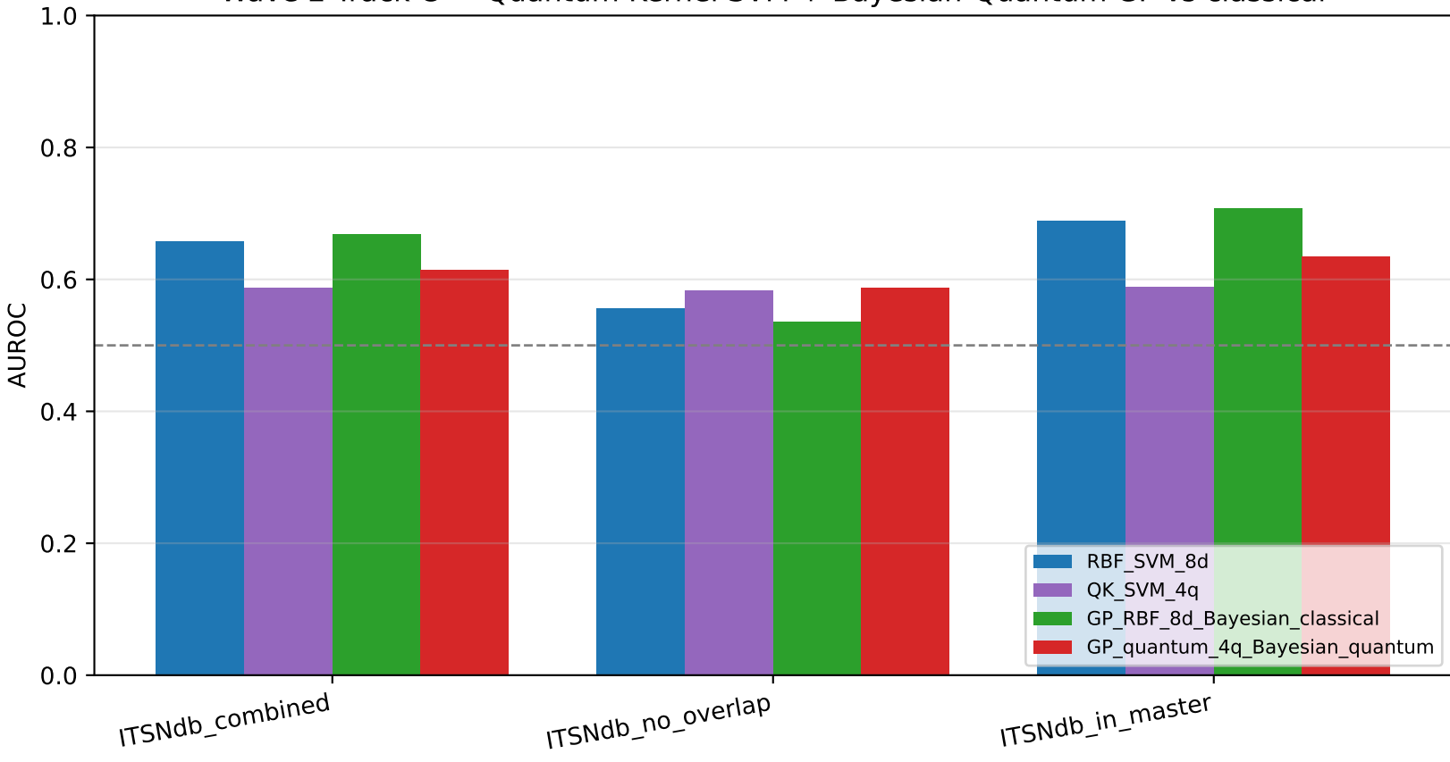
Wave 2 Track C — Quantum Kernel SVM + Bayesian-Quantum GP vs classical
