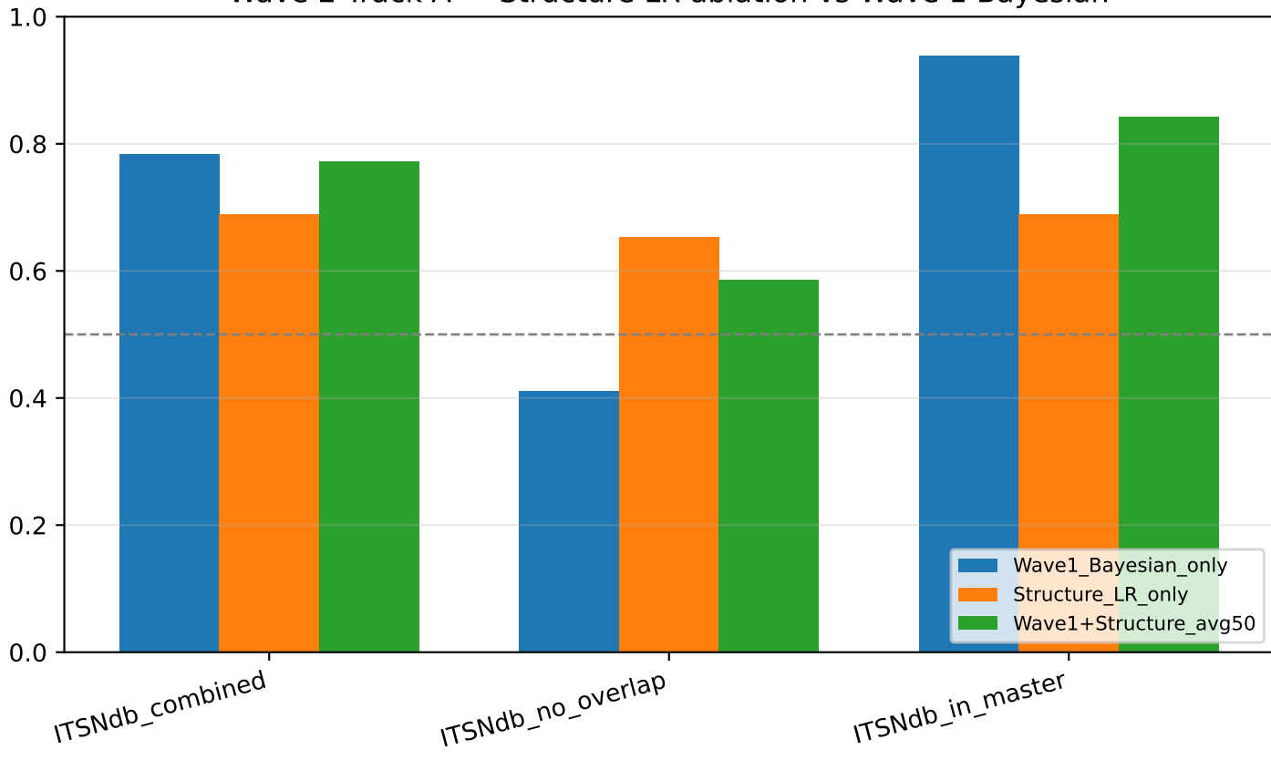
Wave 2 Track A — Structure LR ablation vs Wave 1 Bayesian
