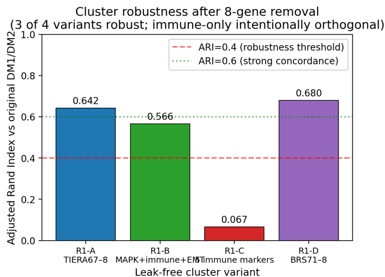
Fig. 9a–c | Cluster robustness across 4 leak-free variants. Top: ARI vs original DM1/DM2 by variant — R1-A/D show strong concordance (0.64/0.68), R1-B moderate (0.57), R1-C orthogonal (0.07, immune axis). Middle: pairwise ARI heatmap between variants. Bottom: cluster sizes per variant.
