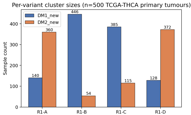
Fig. 9 | Per-variant cluster sizes (n=500 TCGA-THCA primary tumours).
