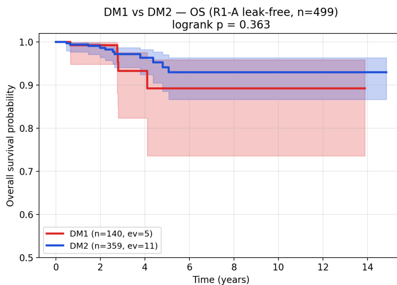
Fig. R6 a-d | DM1/DM2 survival analysis — OS non-significant (TCGA-THCA exceptional-prognosis cohort). a , Full cohort KM ( n = 499 , 16 events; logrank p = 0.363 ). b , Stage III/IV-restricted KM. c , Age \geq 45 KM ( n = 264 , 14 events). d , Combined DM \times TERT 4-group KM (multivariate logrank p = 0.363 ). Plots demonstrate that DM1/DM2 does not provide stage-and-age-independent OS prognostic value in TCGA-THCA’s 3.2% event-rate setting; differentiation axis \neq prognostic axis.
