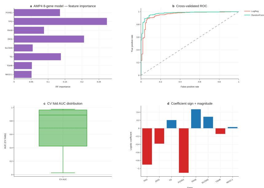
Fig. 6 | AMP4 8-gene RAI decision tool — original (TIERA67) panels. (a) Feature importance (RF). (b) Cross-validated ROC curves. (c) CV-fold AUC distribution. (d) LogReg coefficient sign and magnitude. Panels e–g (DCA, 4-cohort meta, subgroup forest) are moved to Supplement S5–S7 in v6 because they used proxy labels; see leak-free re-validation in Fig. 9 below.
