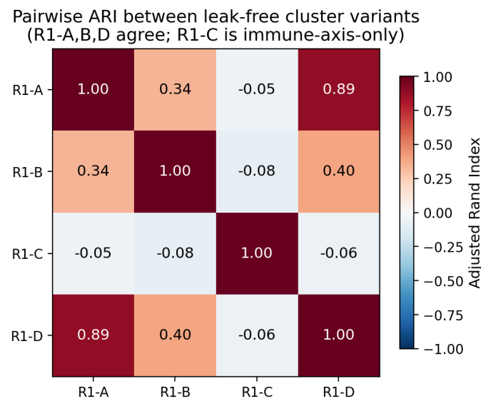
Fig. 9 | Pairwise ARI heatmap between leak-free variants. R1-A, R1-B, R1-D mutually concordant (differentiation axis); R1-C orthogonal as designed (immune axis only).
