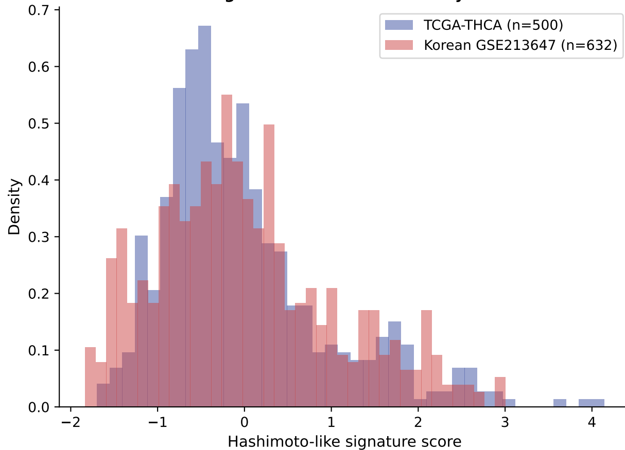
A — Cross-cohort signature distribution overlay
