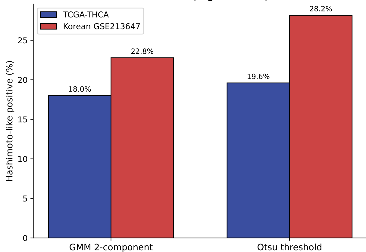
B — Cross-cohort Hashimoto-like prevalence Korean 22-28% \approx TCGA 18-20% (★ generalizes)
