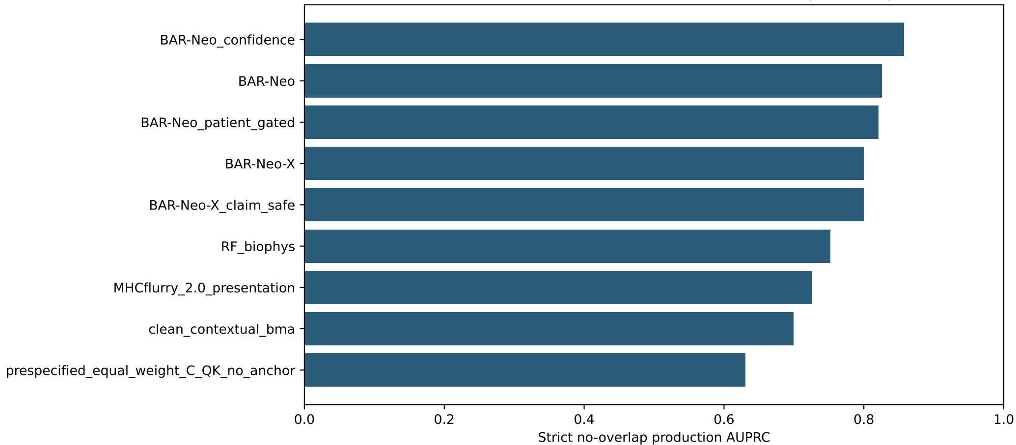
Context caveat: BAR-Neo still wins strict no-overlap reliability
