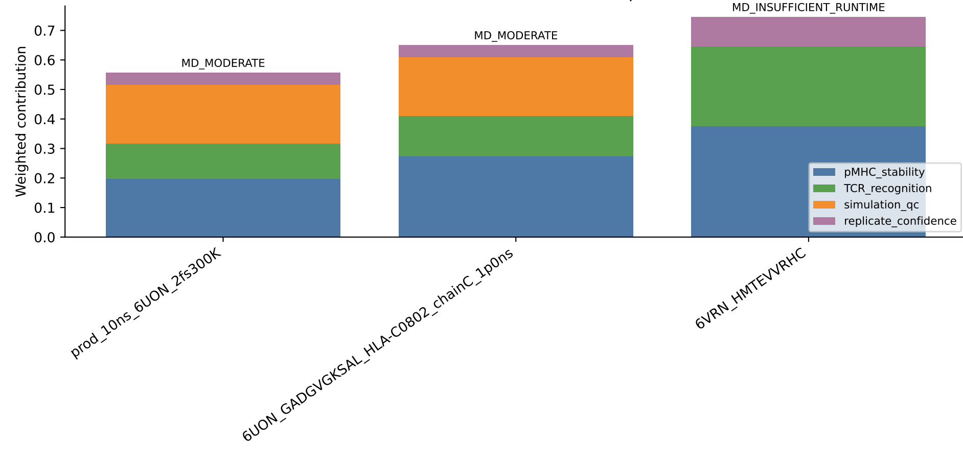
Rule-based MD evidence score components
