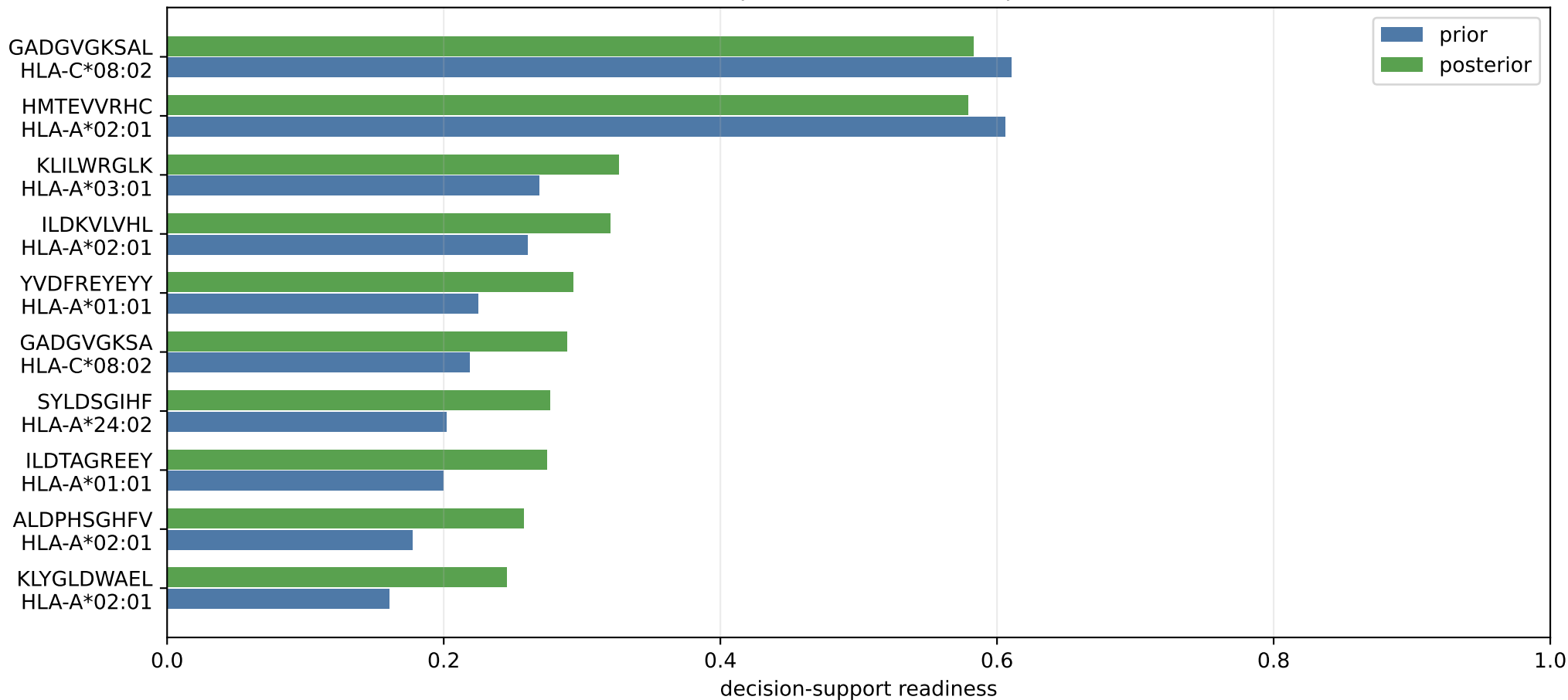
Prior-to-posterior candidate update
