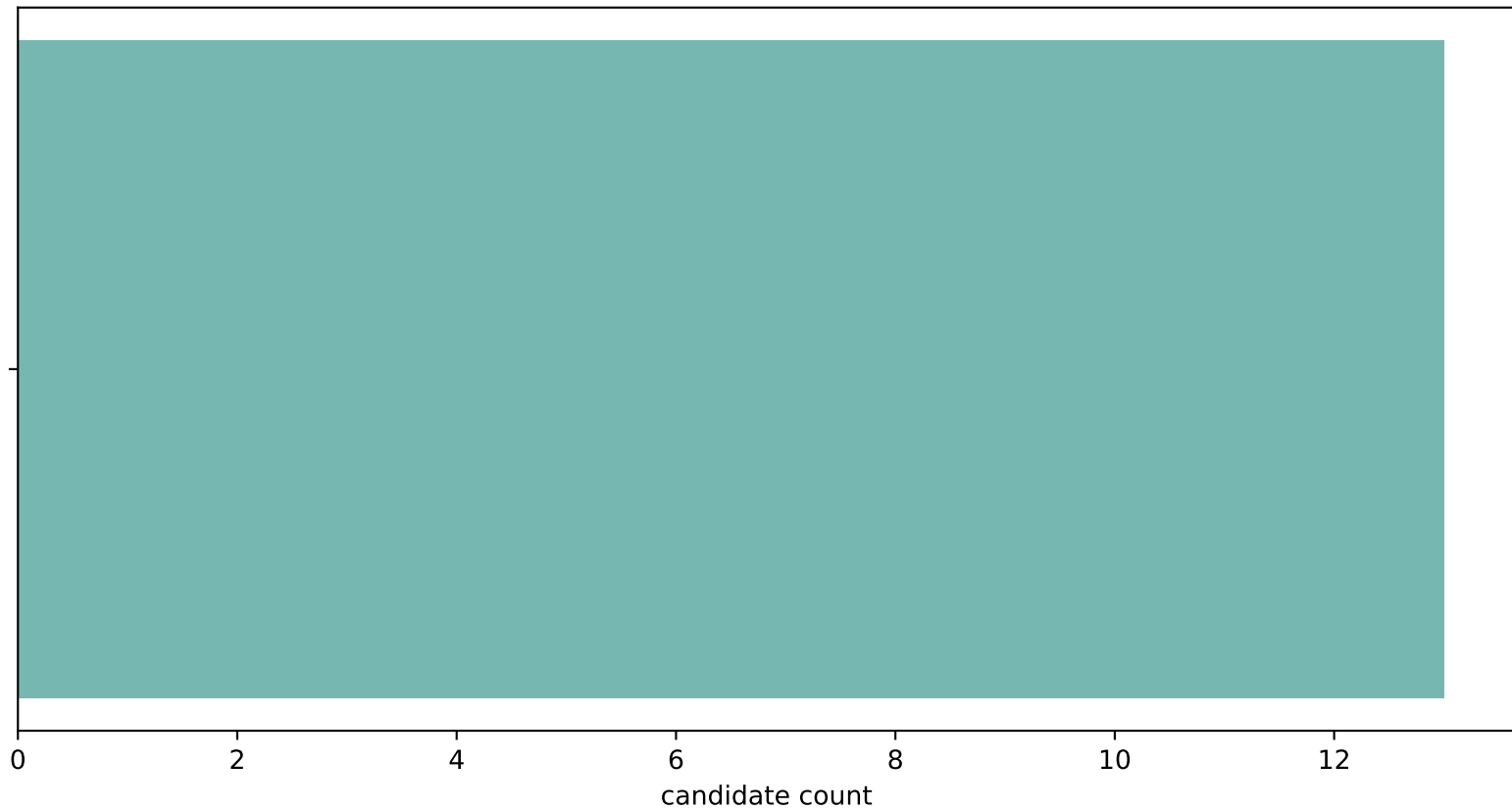
Claim-state distribution
