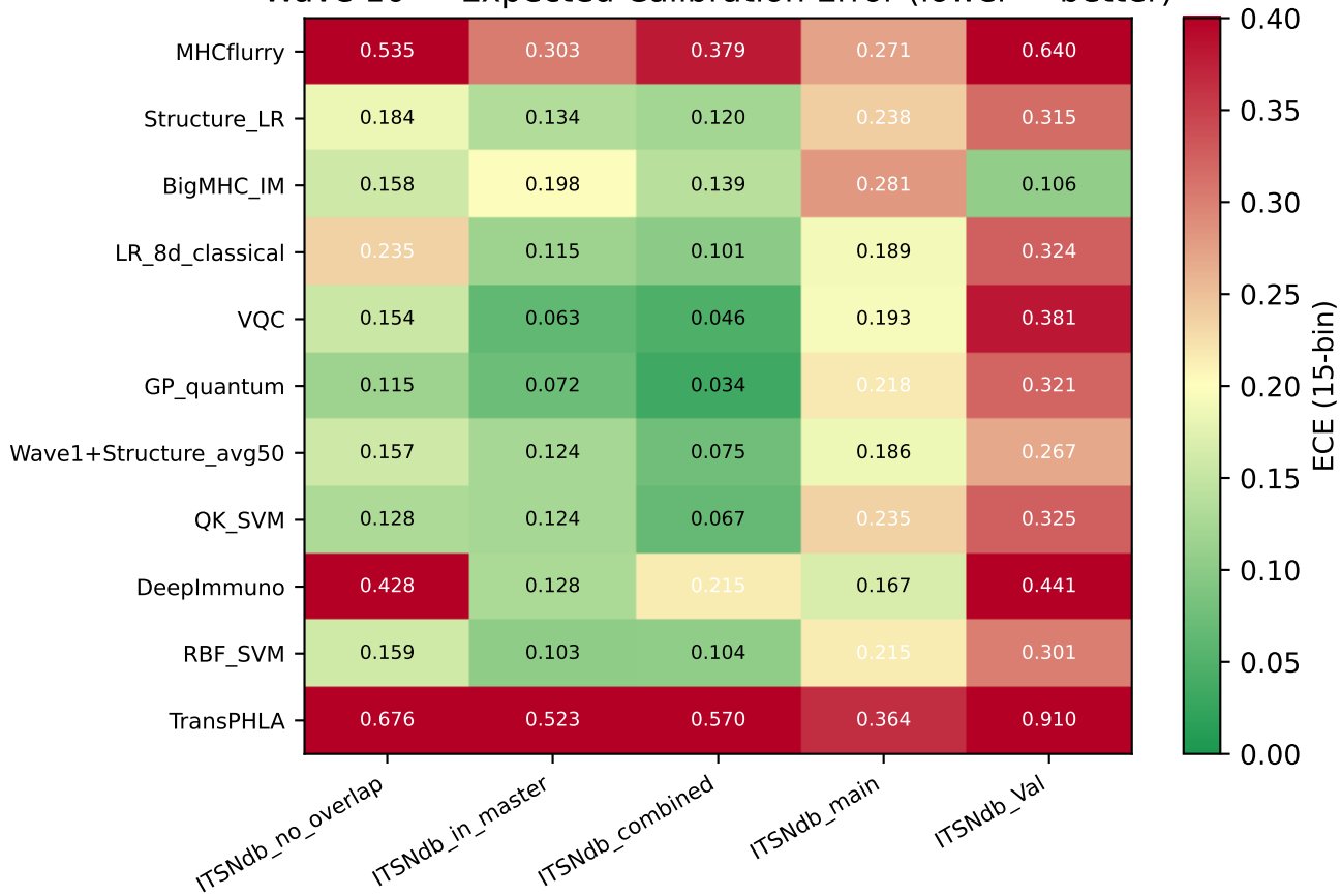
Wave 10 — Expected Calibration Error (lower = better)
